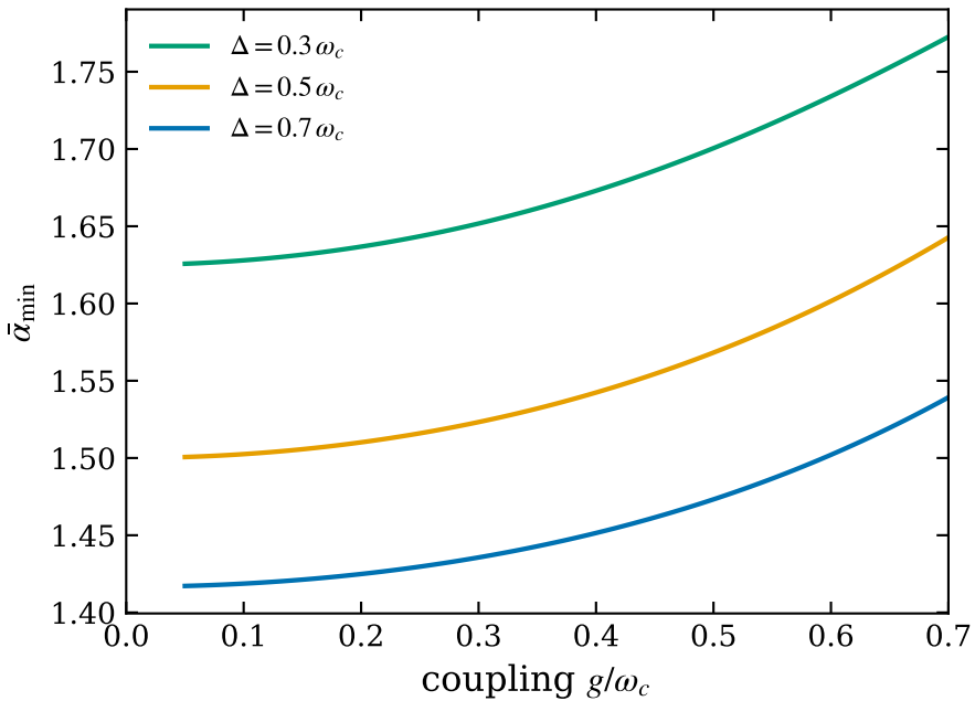
Gauge of minimal photon content \bar{\alpha}_{\min} = 1 - C/2\eta
