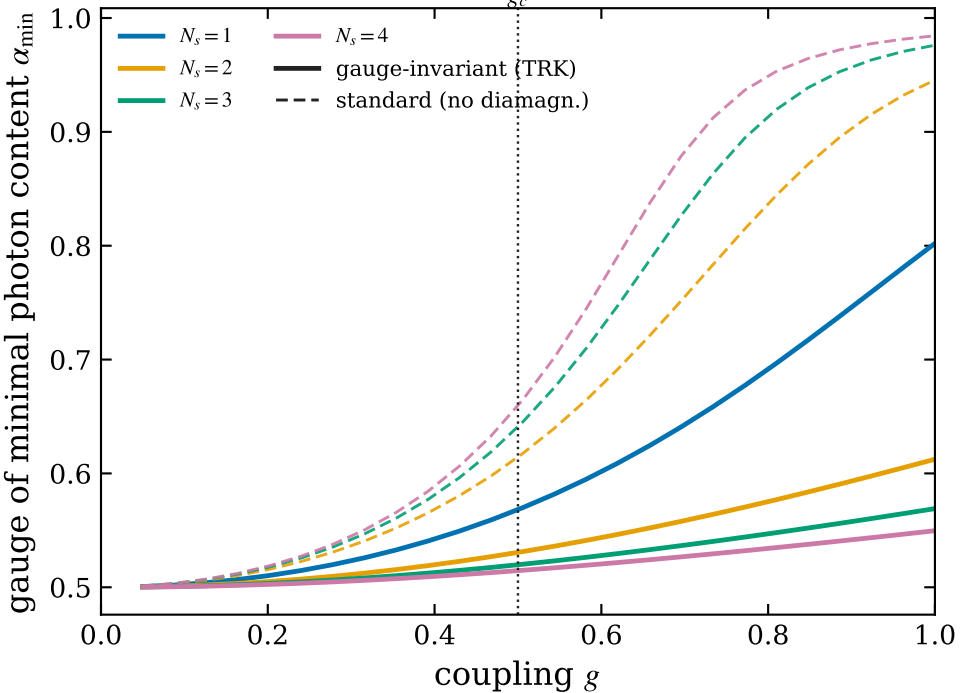
Minimal-photon gauge vs coupling
