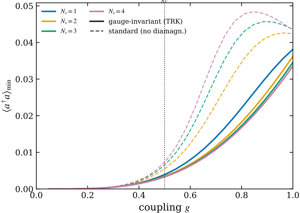
Invariant minimal photon number vs coupling
