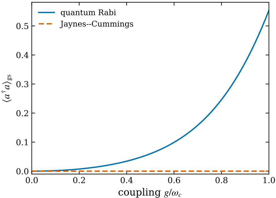
Ground-state photon number, \Delta = 0.7 \omega_c
