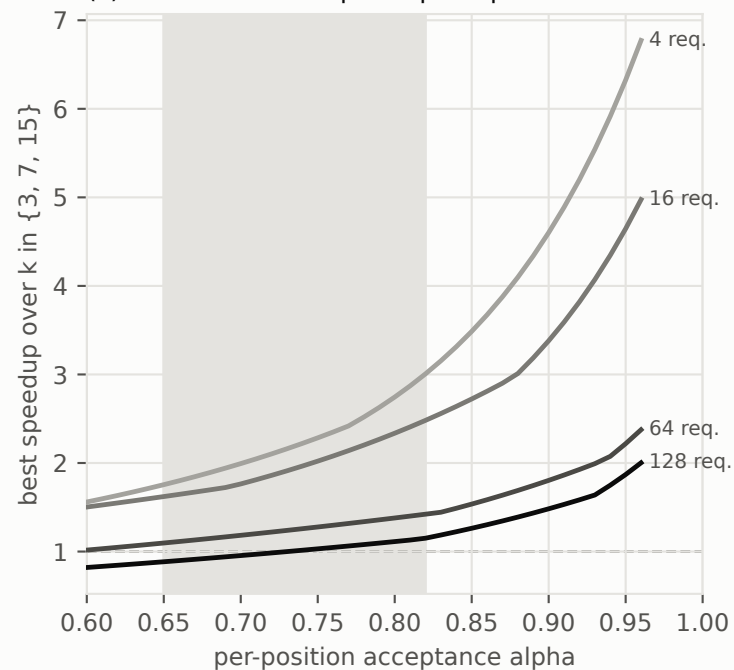
(c) Gemma 4 31B: speedup if alpha were raised
