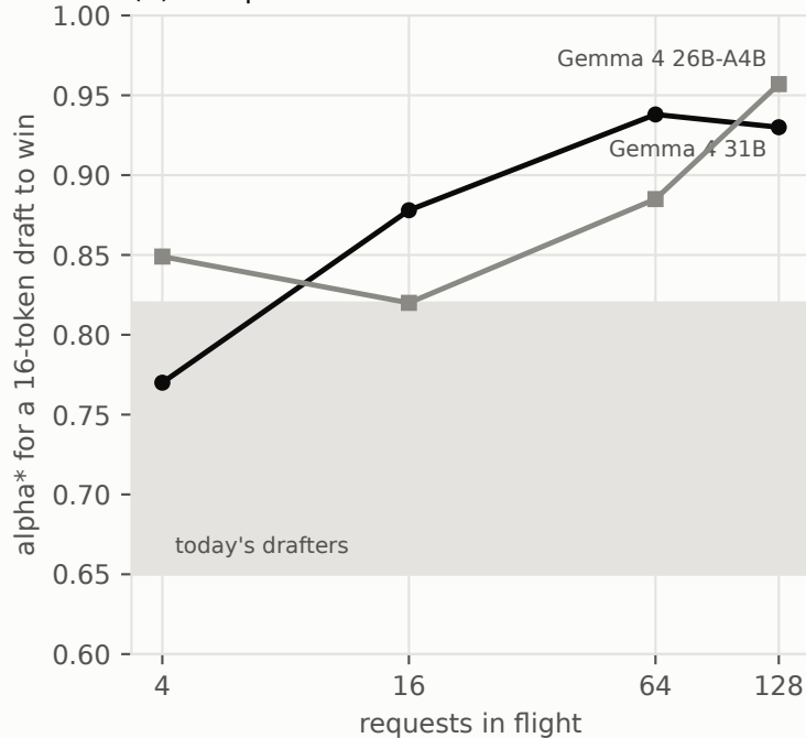
(b) acceptance needed rises with load
