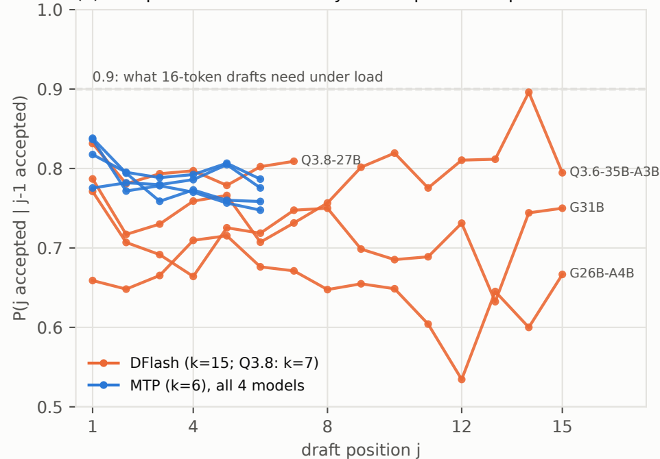
(a) acceptance does not decay with depth: it compounds
