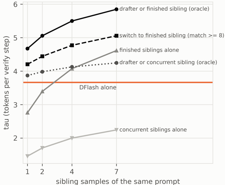
(b) Gemma 4 31B, T = 1: acceptance rises with siblings
