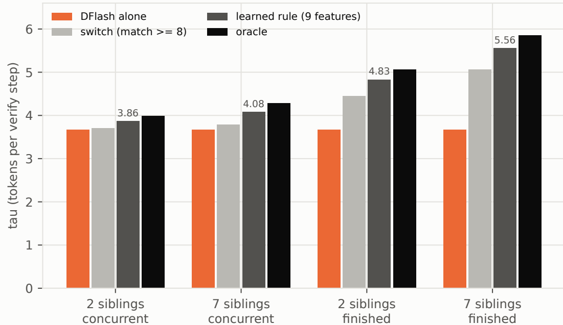
(a) a cheap learned rule recovers most of the oracle gain
