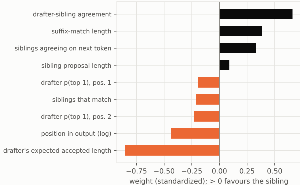
(b) what the rule looks at (7 finished siblings)
