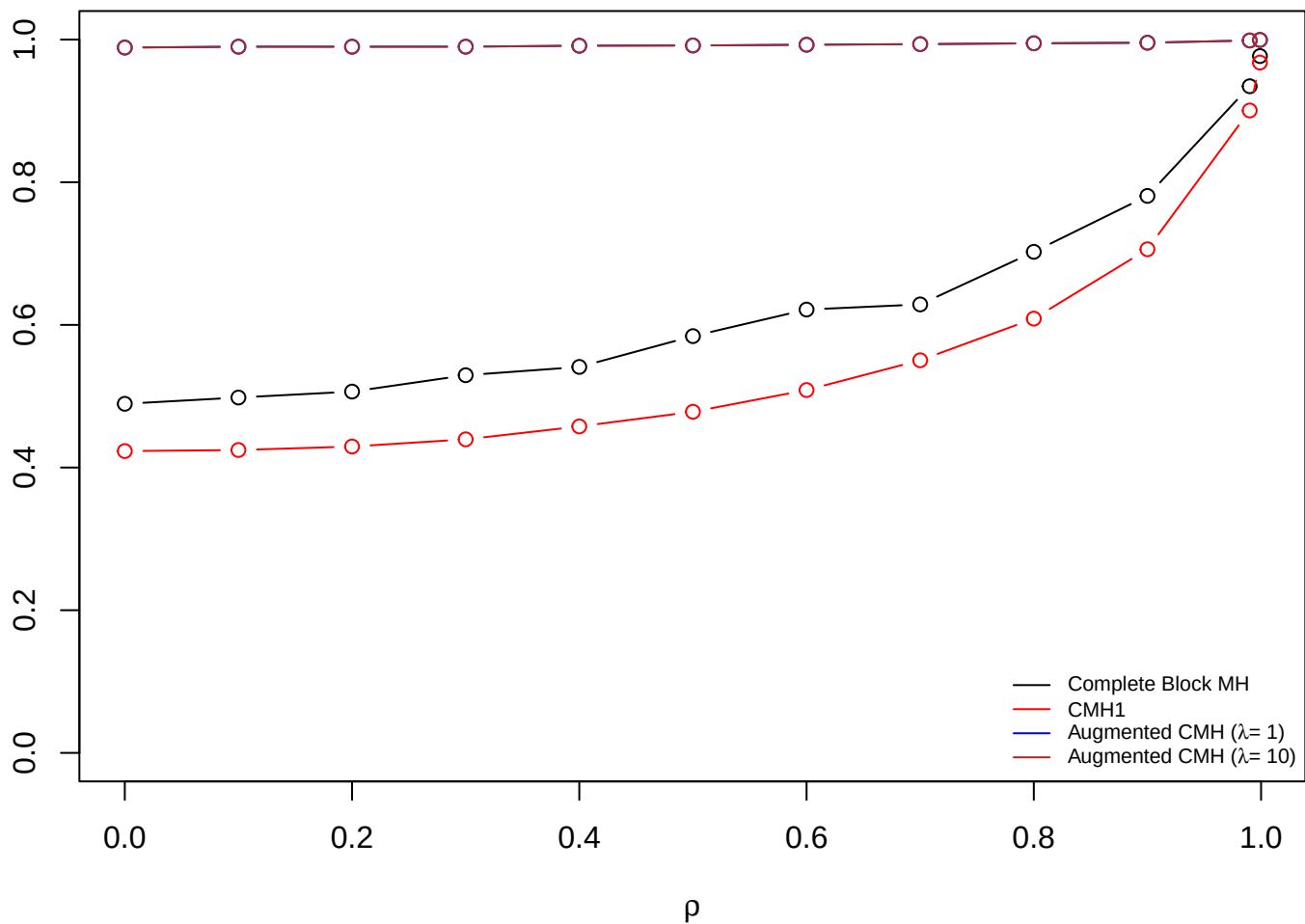
Estimated Lower Bounds
