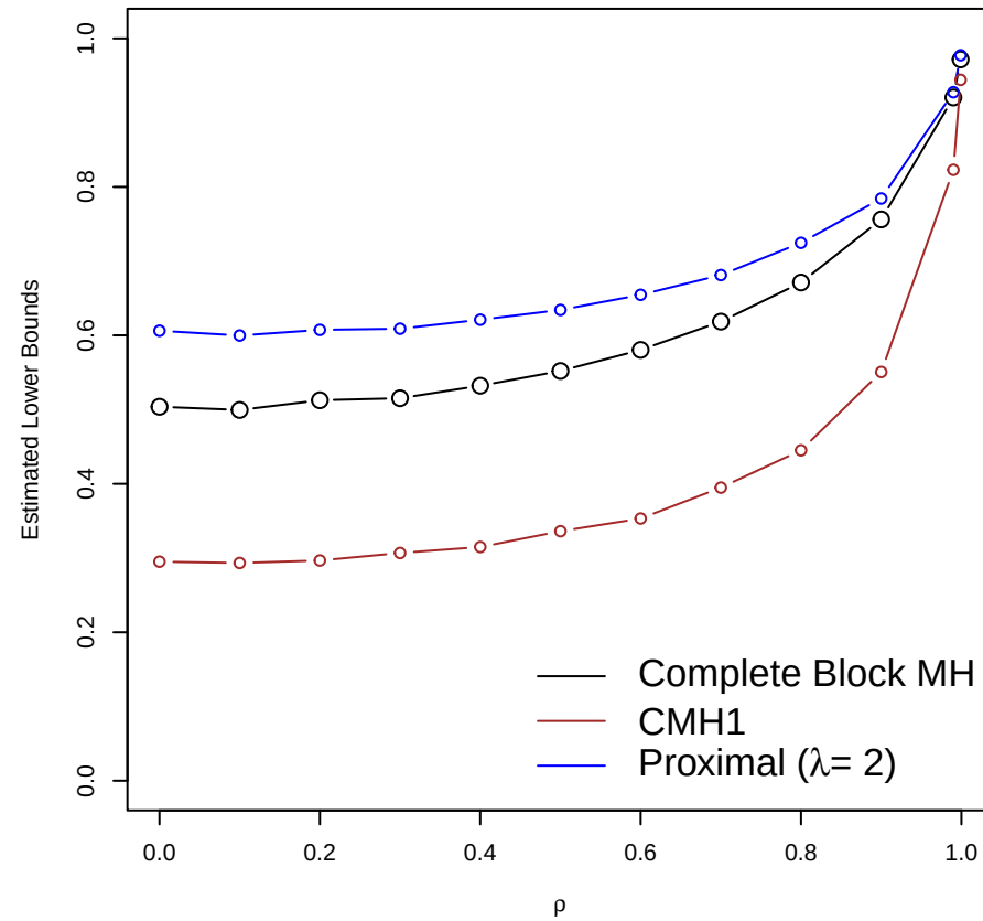
h = 1
