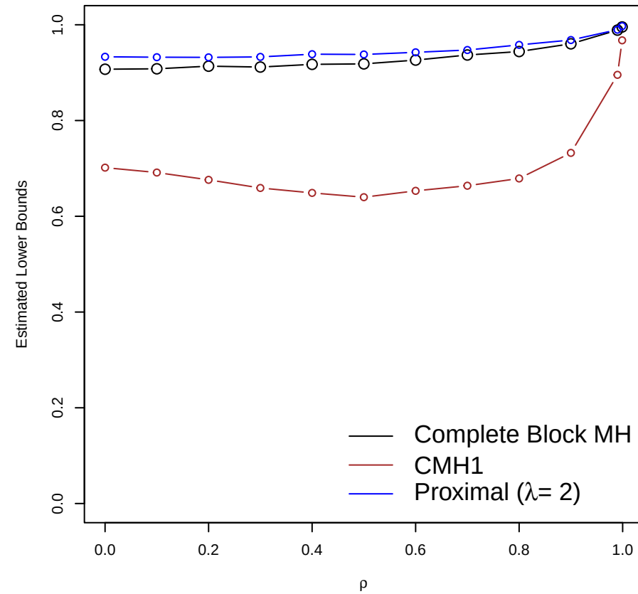
h = 10
