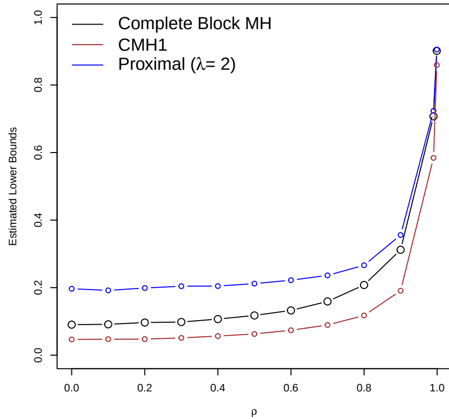
h = 0.1
