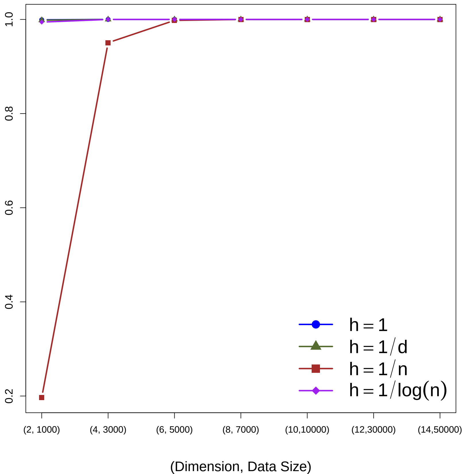
Lower Bounds
