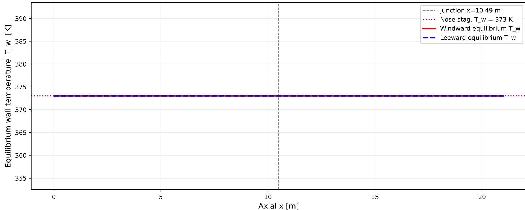
Radiation-Equilibrium Wall Temperature — Body M=5.0, h=30 km, AoA=1.0°, Turb. BL, Cold-wall Tw=373 K
