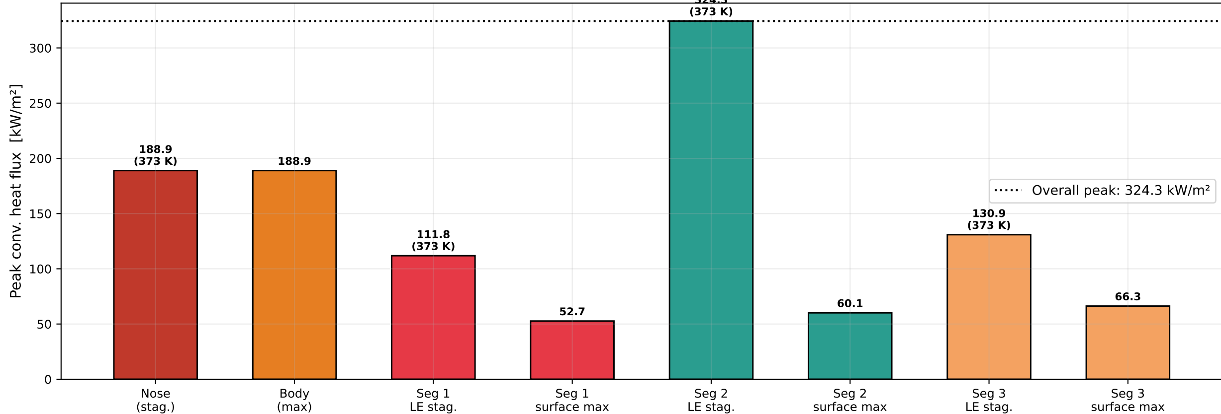
Peak Heat Flux per Component — TPS Sizing Reference M=5.0, h=30 km, AoA=1.0°, Turb. BL, Cold-wall Tw=373 K
