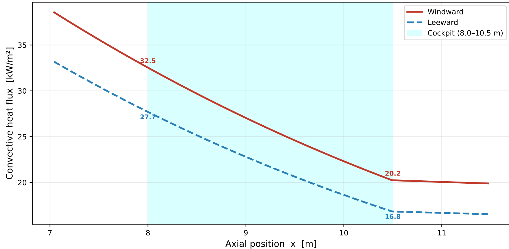
Cockpit Region Heat Flux Detail M=5.0, h=30 km, AoA=1.0°, Turb. BL, Cold-wall Tw=373 K
