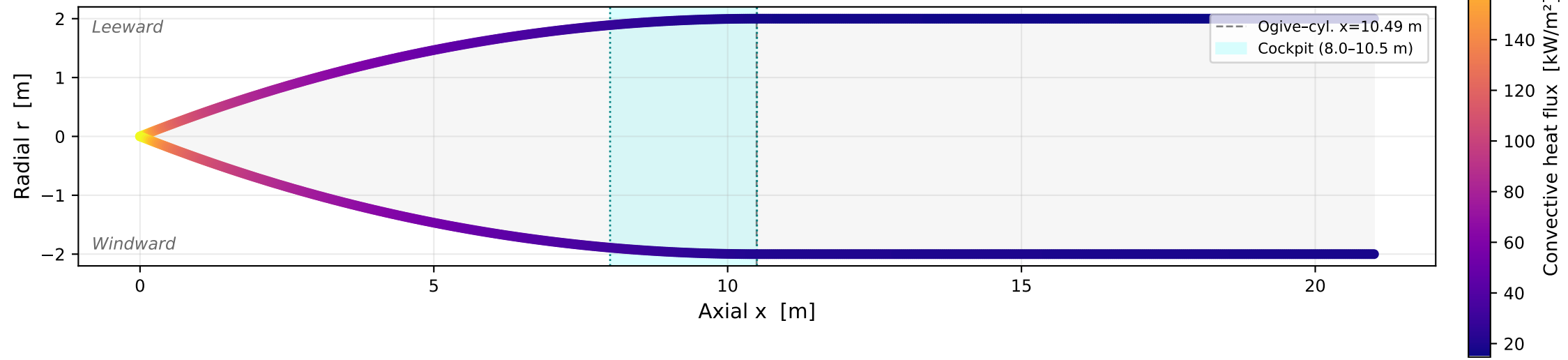
Thermal Landscape (windward + leeward) — M=5.0 , h=30 km, AoA=1.0^\circ , Turb. BL, Cold-wall T_w=373 K
