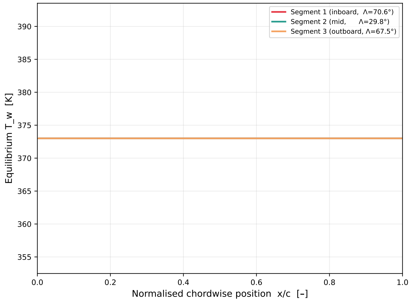
Upper (leeward) surface equilibrium wall temperature
