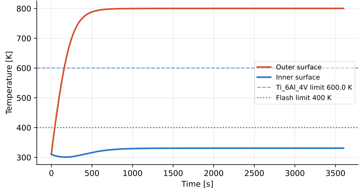
Heat Soak into Ti_6Al_4V Layer
