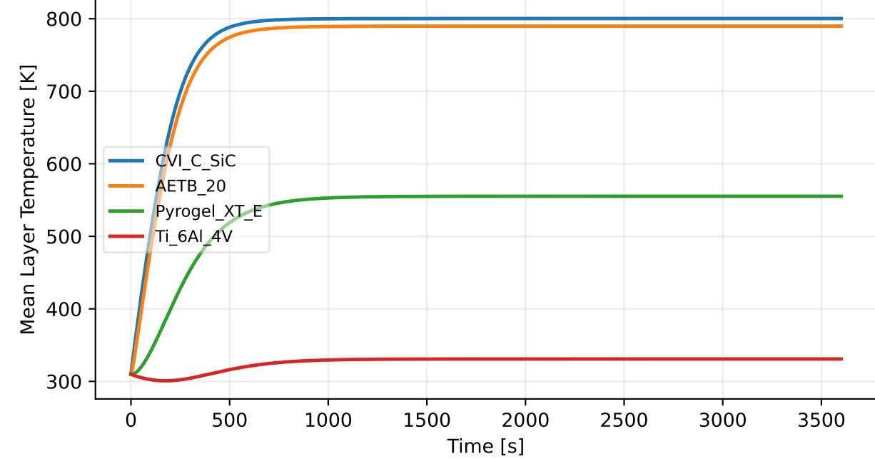
Layer-Average Temperatures
