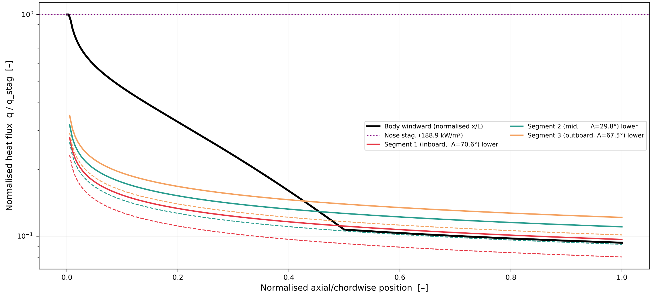
Normalised Convective Heat Flux ( q / q_{\text{stag}} ) M=5.0, h=30 km, AoA=1.0°, Turb. BL, Cold-wall Tw=373 K
