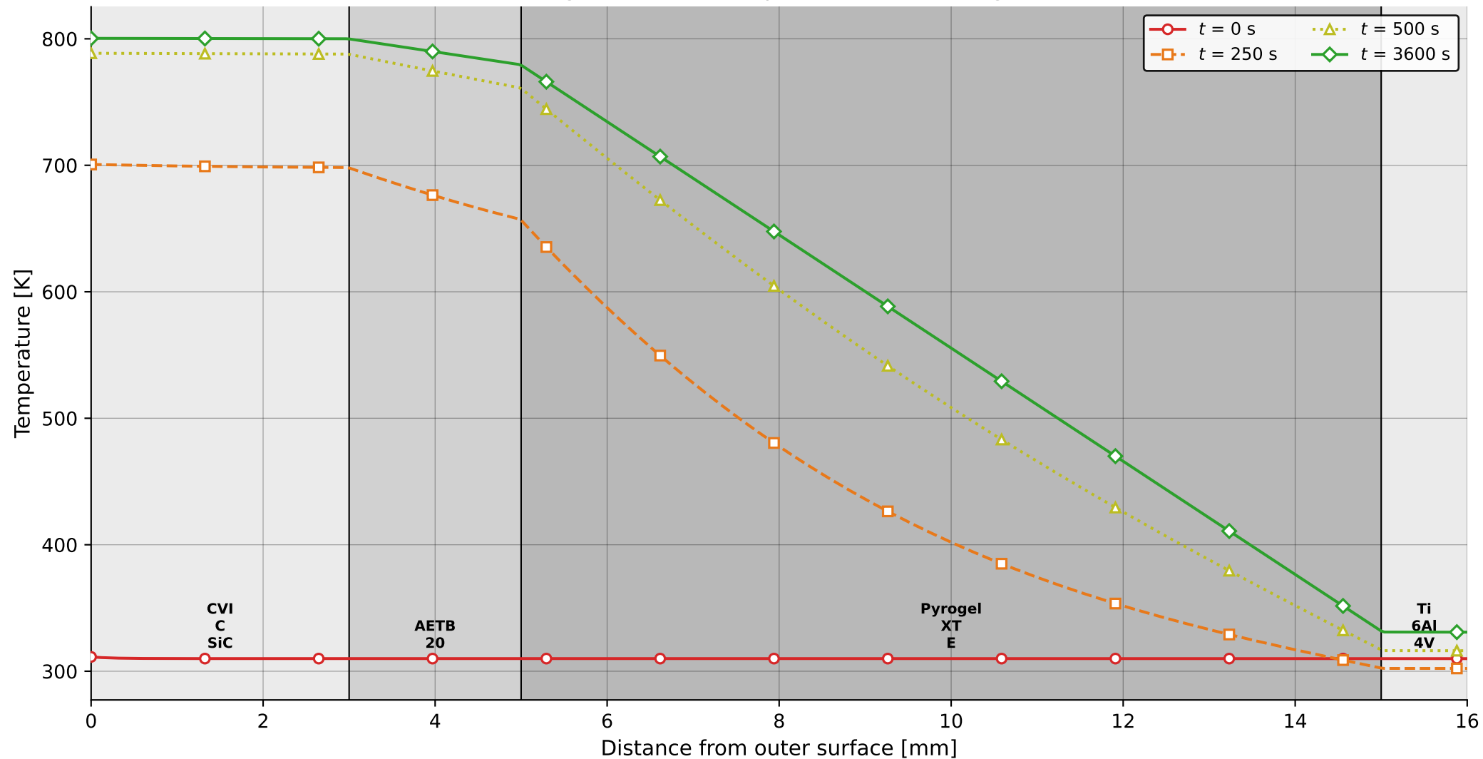
Through-Thickness Temperature Profile Wing Skin
