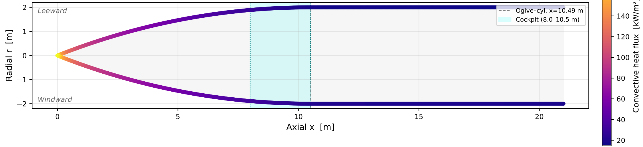
Thermal Landscape (windward + leeward) — M=5.0 , h=30 km, AoA=1.0^\circ , Turb. BL, T_w=373 K
