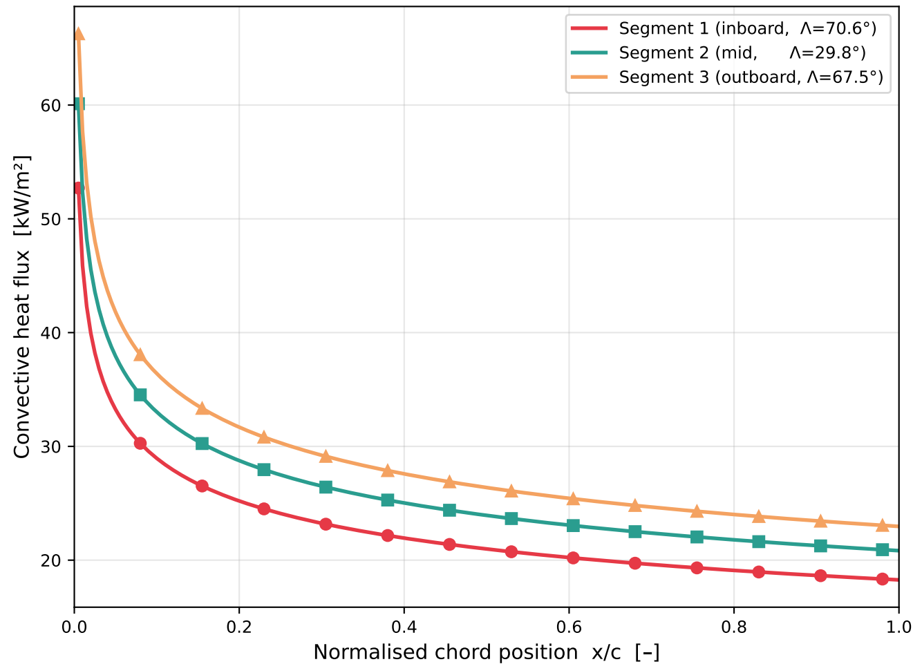
Lower Surface (windward)
