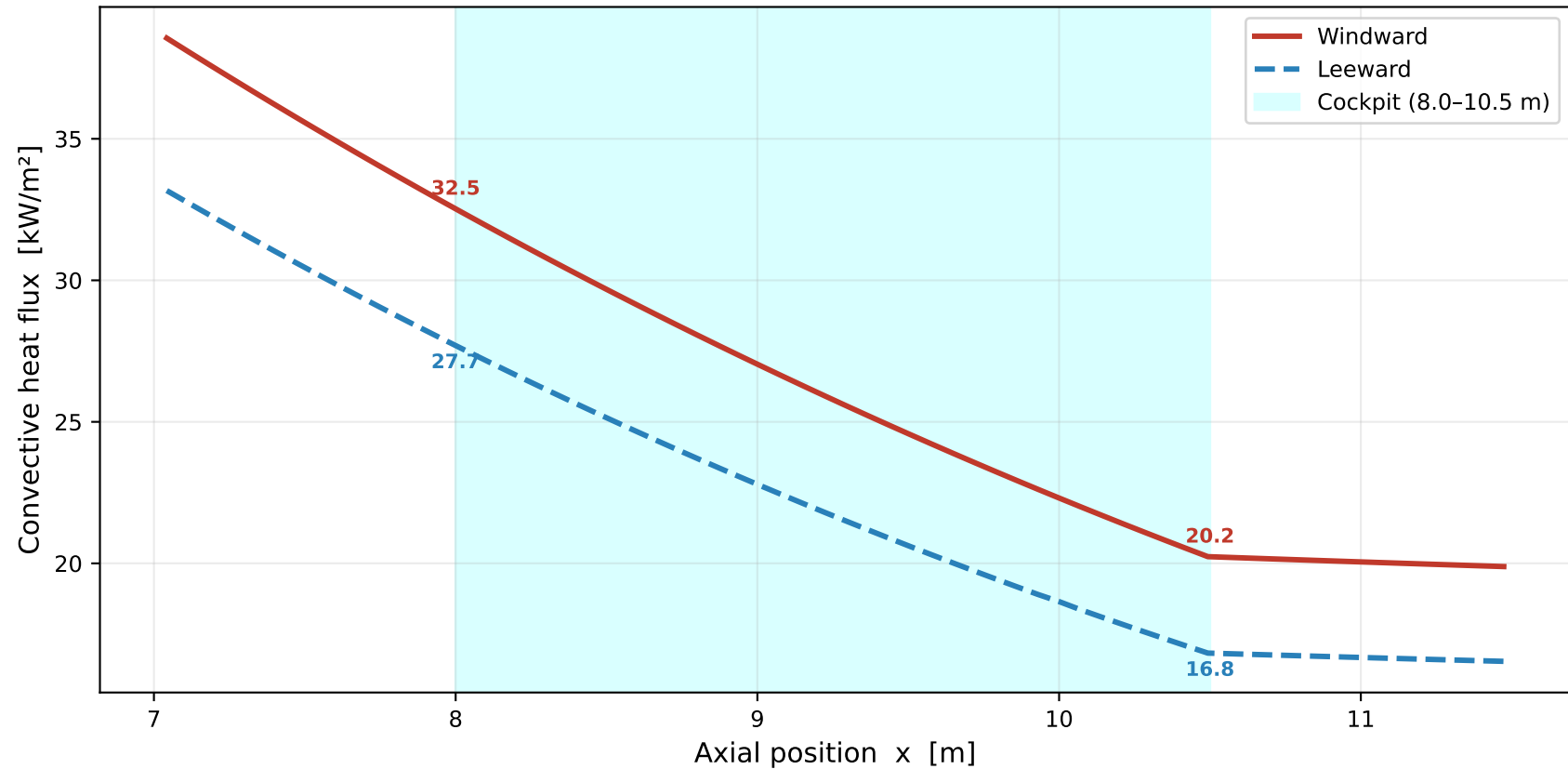
Cockpit Region Heat Flux Detail M=5.0, h=30 km, AoA=1.0°, Turb. BL, Tw=373 K
