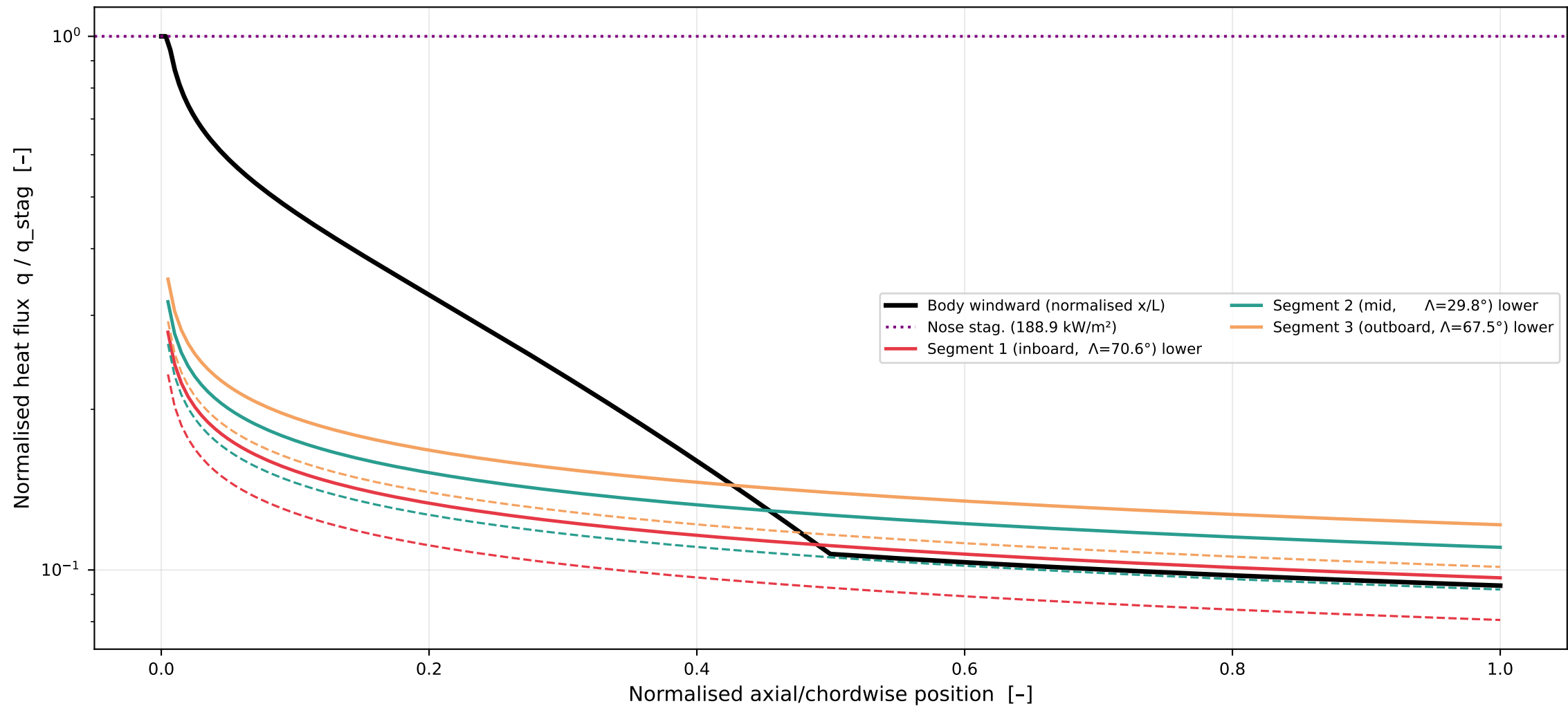
Normalised Convective Heat Flux ( q / q_{\text{stag}} ) M=5.0, h=30 km, AoA=1.0°, Turb. BL, Tw=373 K
