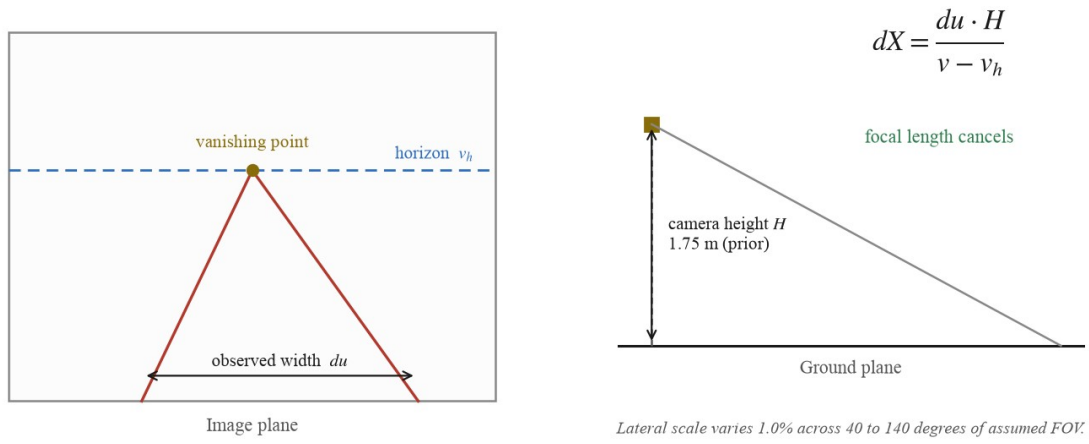
Figure 6. Recovering metric scale from the vanishing point.
