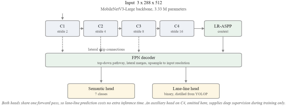
Figure 5. Segmentation network architecture.
