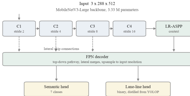
Figure 5. Segmentation network architecture.
