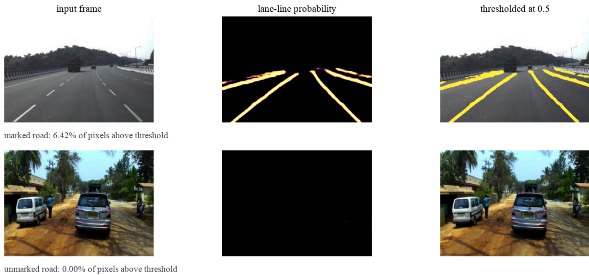
Figure 8. The distilled lane marking head on a marked and an unmarked road.
