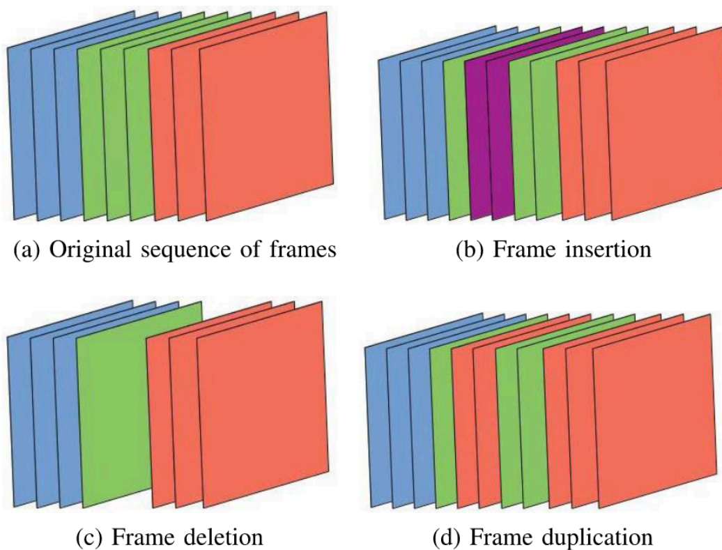
Figure 9: Modification of GOP structure [2]
