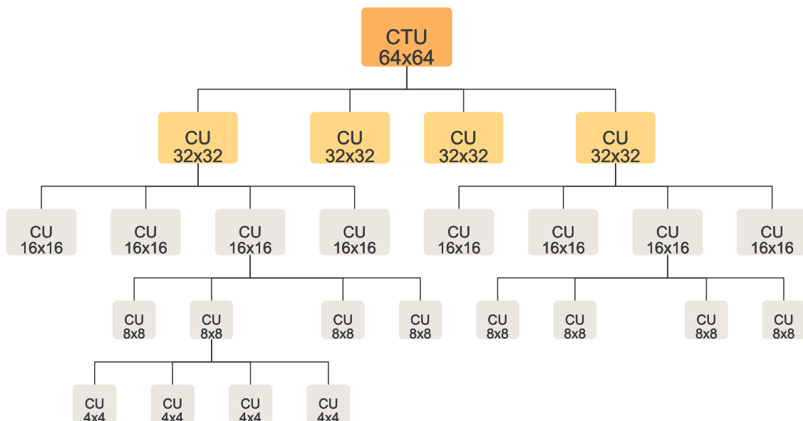
Listing 1: Structure of H265 code
