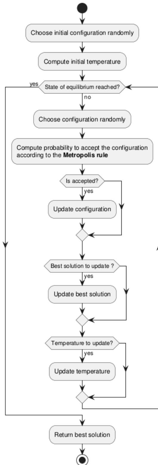
Figure 2: Simulated Annealing Diagram
