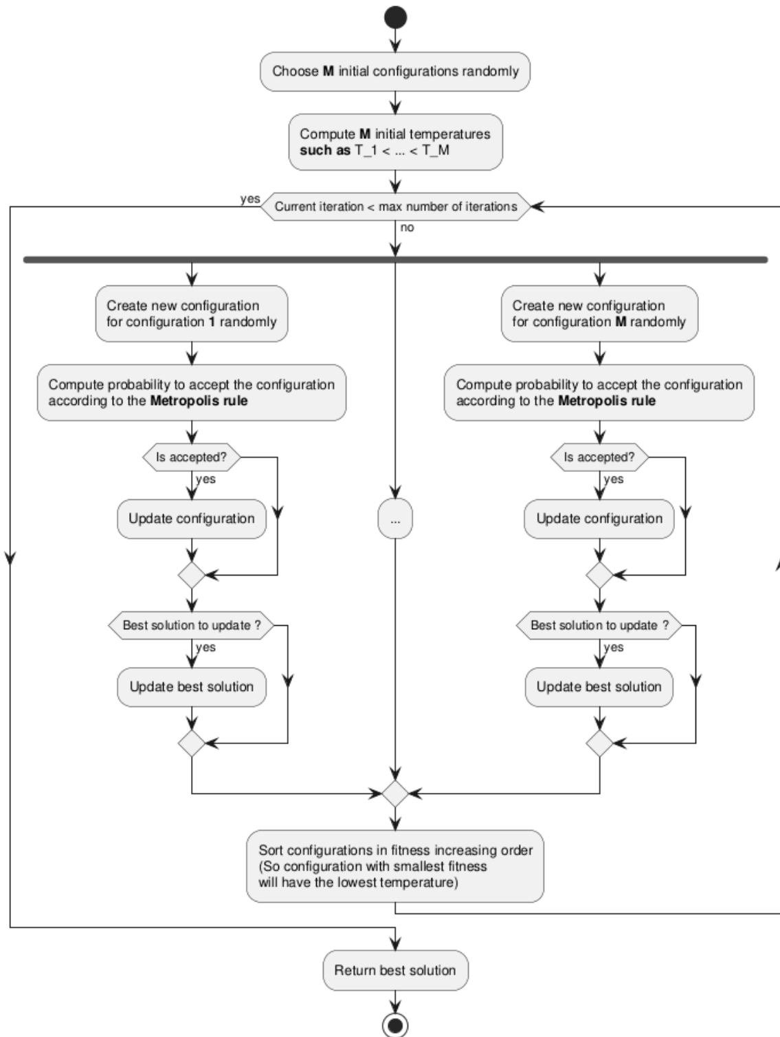
Figure 3: Parallel Tempering Diagram
