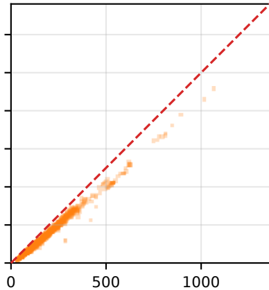
Qwen3.5-35B-A3B
