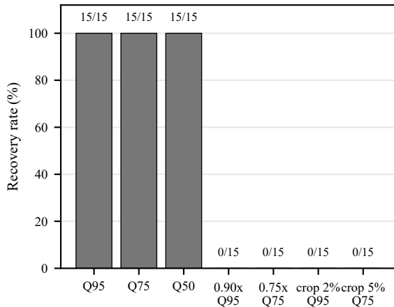
Controlled offline transforms of retained Phase 3 stego JPEGs
