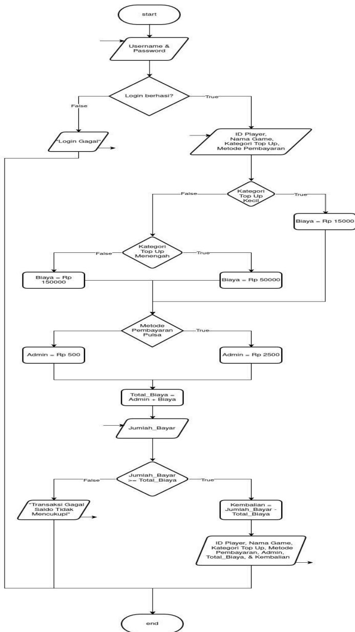
Gambar 1.1 FlowChart
