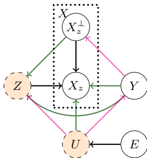
(a) \mathcal{G}_1 : anti-causal
