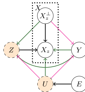
(c) \mathcal{G}_3 : confounded-outcome
