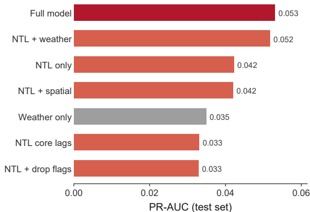
C Feature-family ablation
