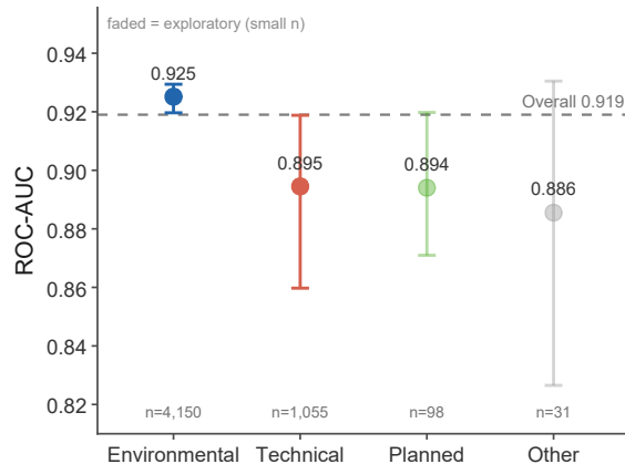
D Cause-stratified ROC-AUC (test set, 95% CI)
