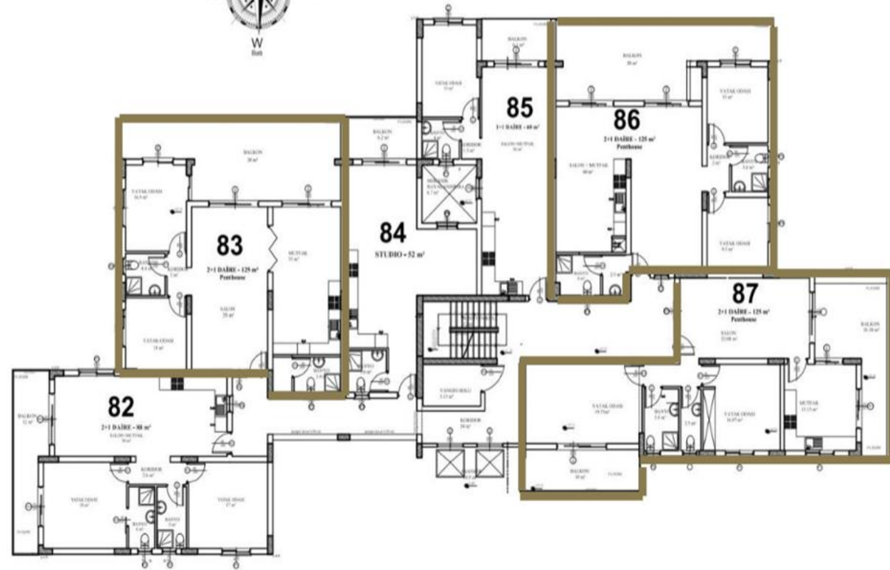
VENICE FLOOR PLAN FLOOR - 9
