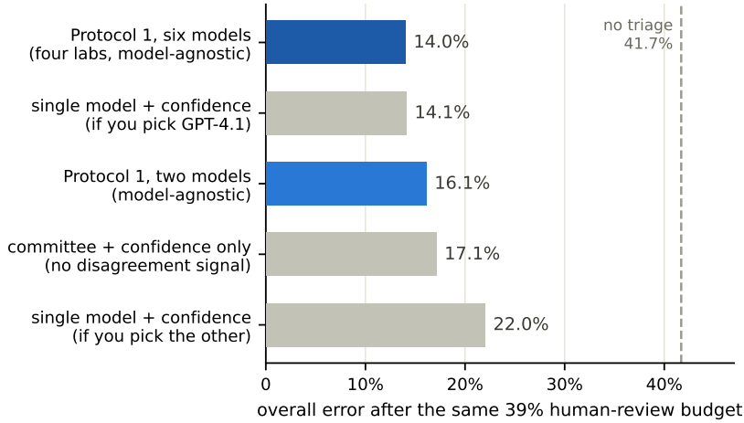
Figure 2: End-to-end protocol effectiveness: overall error after spending the same 38.7% human-review budget under each strategy (baseline condition, humans assumed correct; dashed line = no triage). The two-model protocol beats confidence-only routing of the same committee and every ex-ante single-model strategy; the six-model, four-lab variant matches the hindsight-best single model without the hindsight. Reproduced by analysis/fig-protocol-e2e.py .
