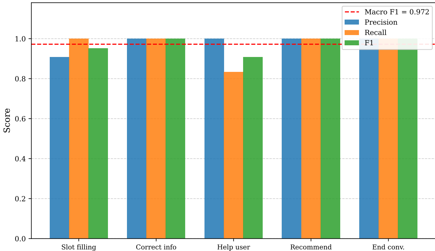
Action Selection — Per-action Precision, Recall, F1
