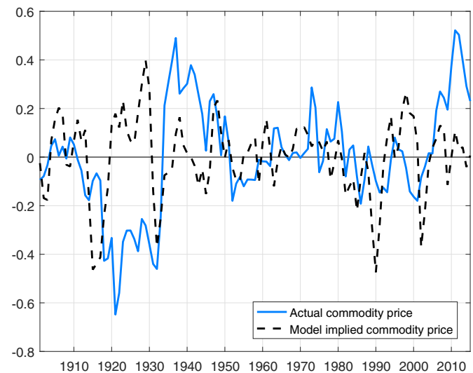
Fig. 7. Estimated and actual process for commodity prices.
