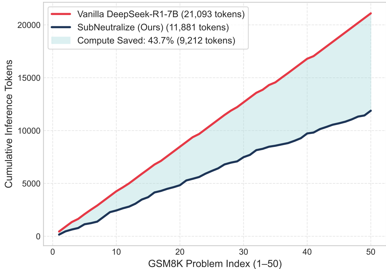
A. Cumulative Test-Time Compute on NVIDIA A100
