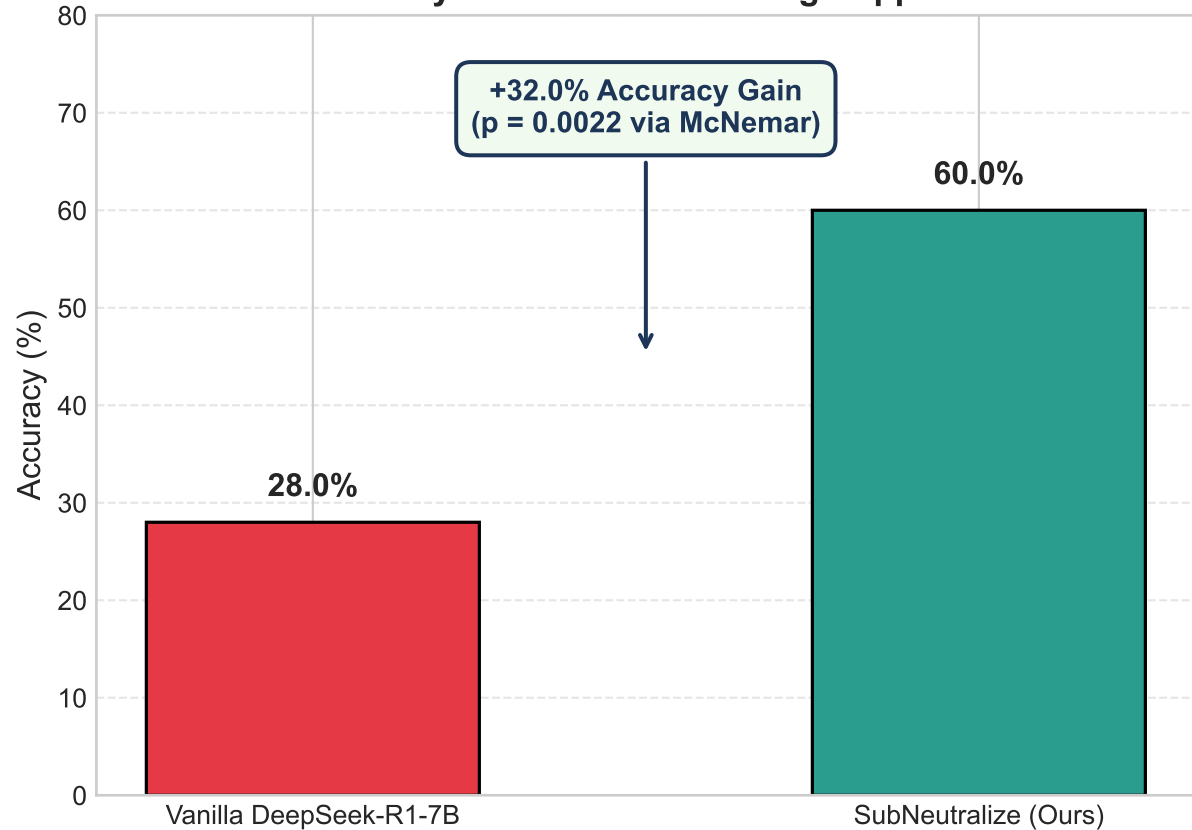
B. Accuracy Gain via Overthinking Suppression
