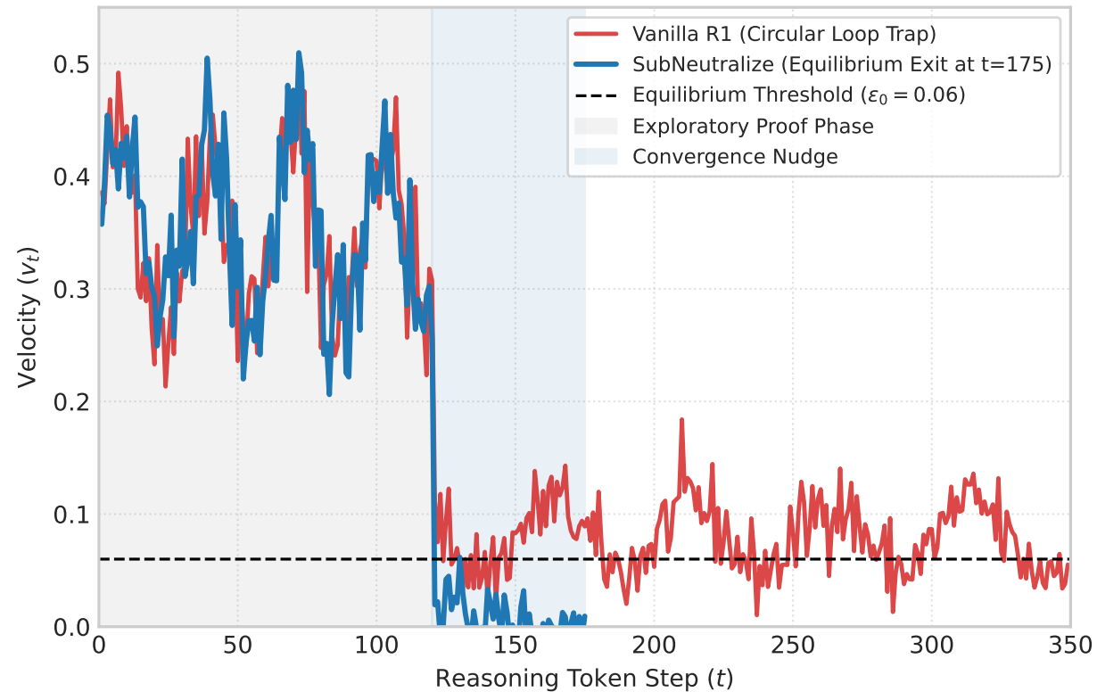
(a) Riemannian Trajectory Velocity ( v_t = 1 - \cos )
