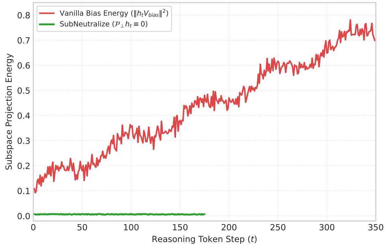
(b) Prompt Bias Subspace Energy Dynamics
