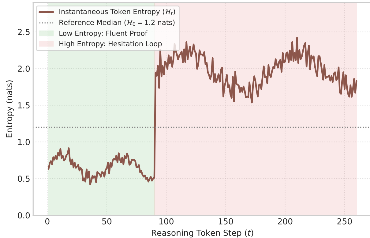
(a) Instantaneous Shannon Entropy \mathcal{H}_t
