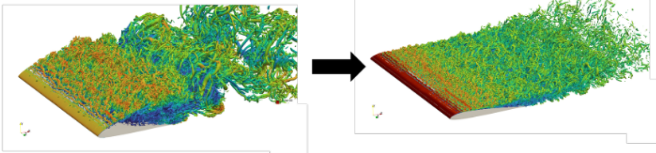
SD 7003 – Re = 60,000 (16M DoFs / 4 GPUs)
