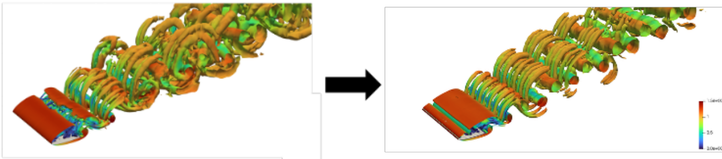
SD 7003 – Re = 60,000 (16M DoFs / 4 GPUs)
