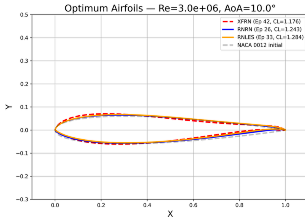
(a) Optimum Airfoils
