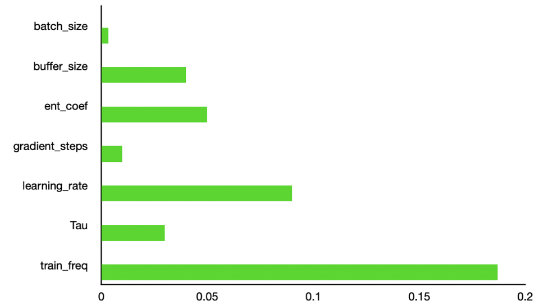
(b) Hyper-parameter importance
