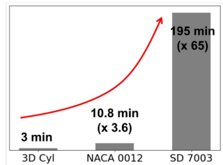
Wall-Time / Episode [min]
