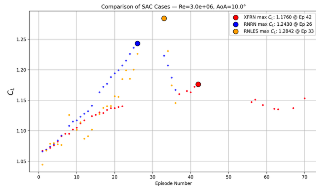
(b) Lift Evaluation (Deterministic)
