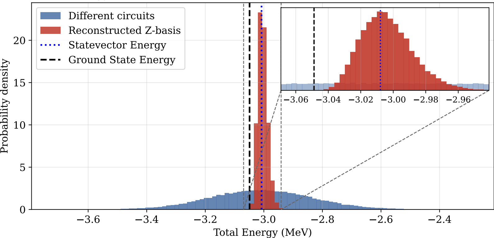
Total Energy Distribution of {}^6\text{Be}
