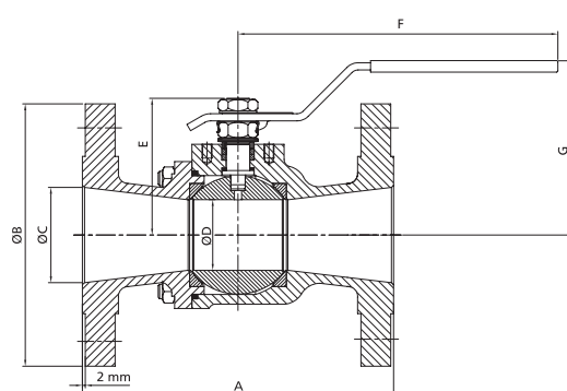
Lever operated (DN 50 & DN 65)
