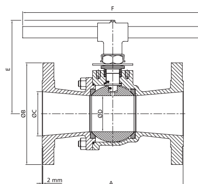
Wrench operated (DN 80 - DN 200)
