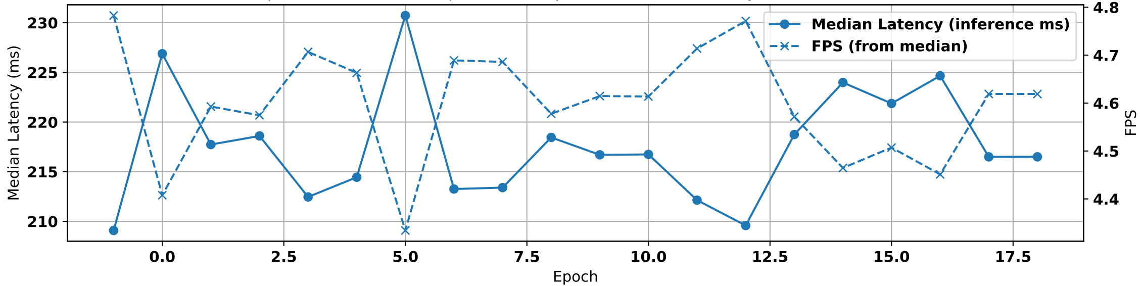
UnpretrainedYOLO — Speed over Epochs (median latency = inference ms)
