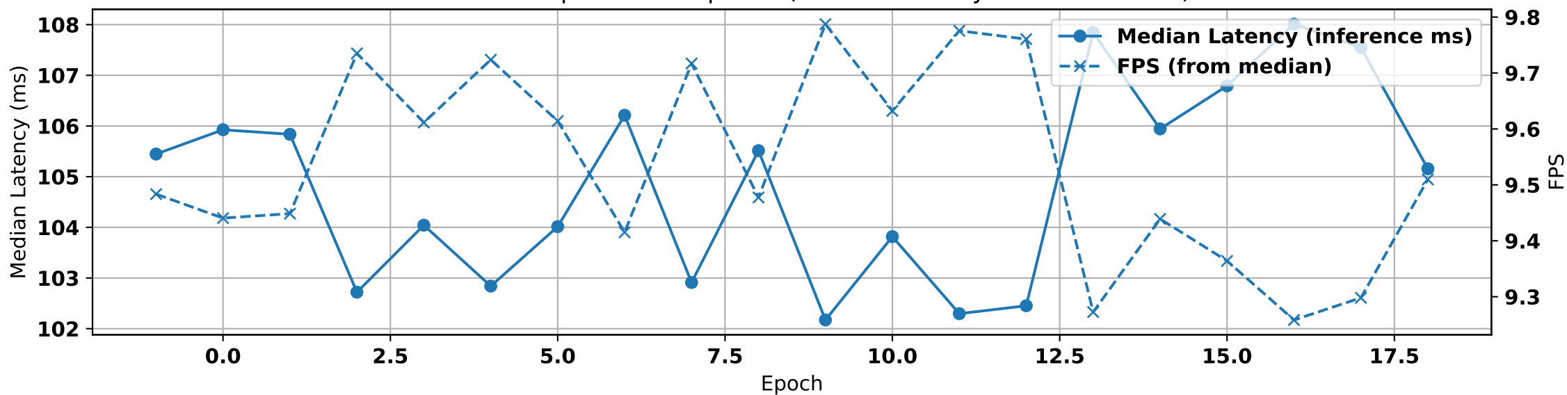
FastYOLO — Speed over Epochs (median latency = inference ms)
