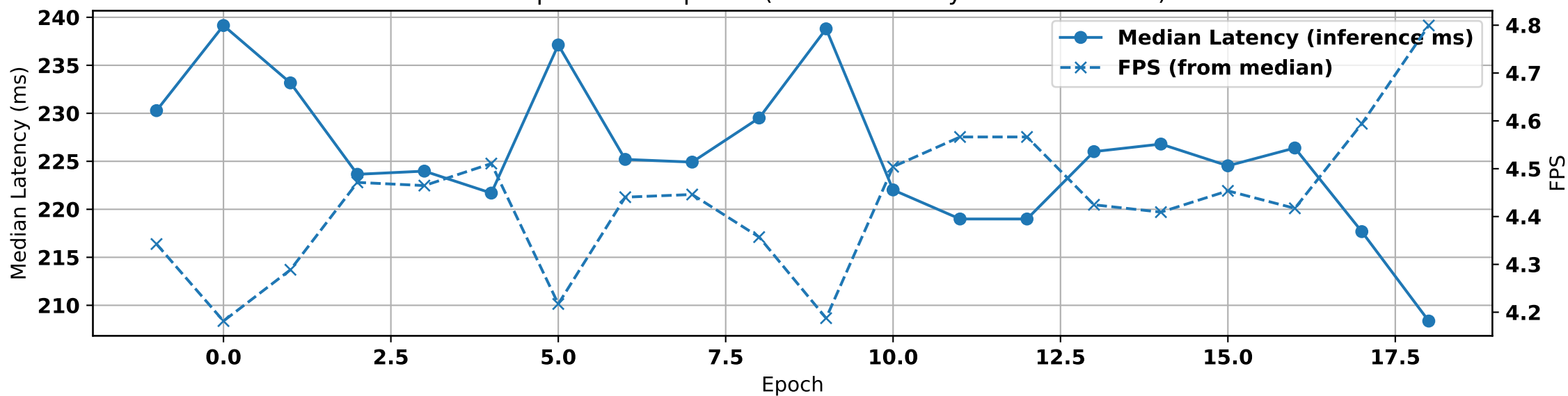
YOLO — Speed over Epochs (median latency = inference ms)
