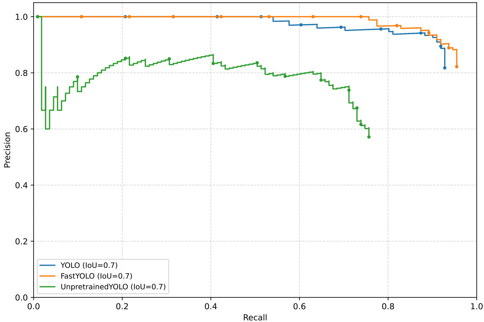
Precision — Recall curves at IoU = 0.70
