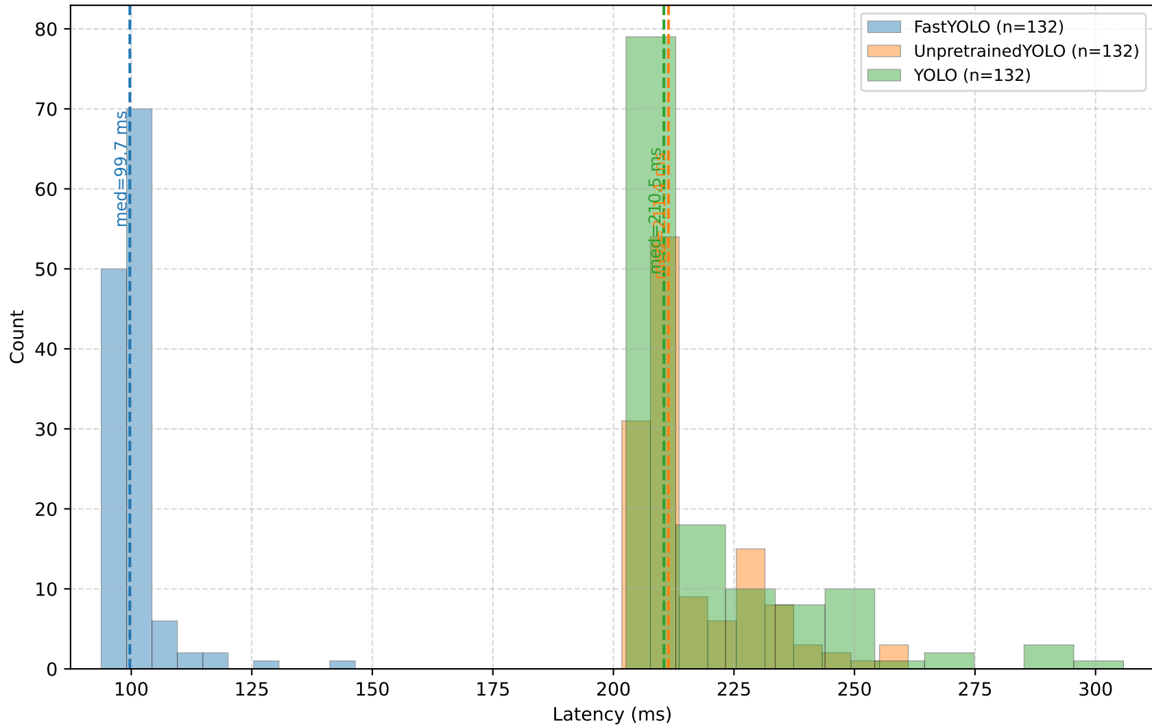
Validation Latency Histograms (ms) — per-model
