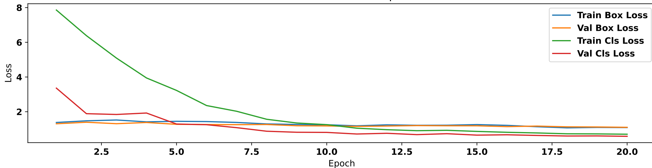
FastYOLO — Metrics over Epochs
