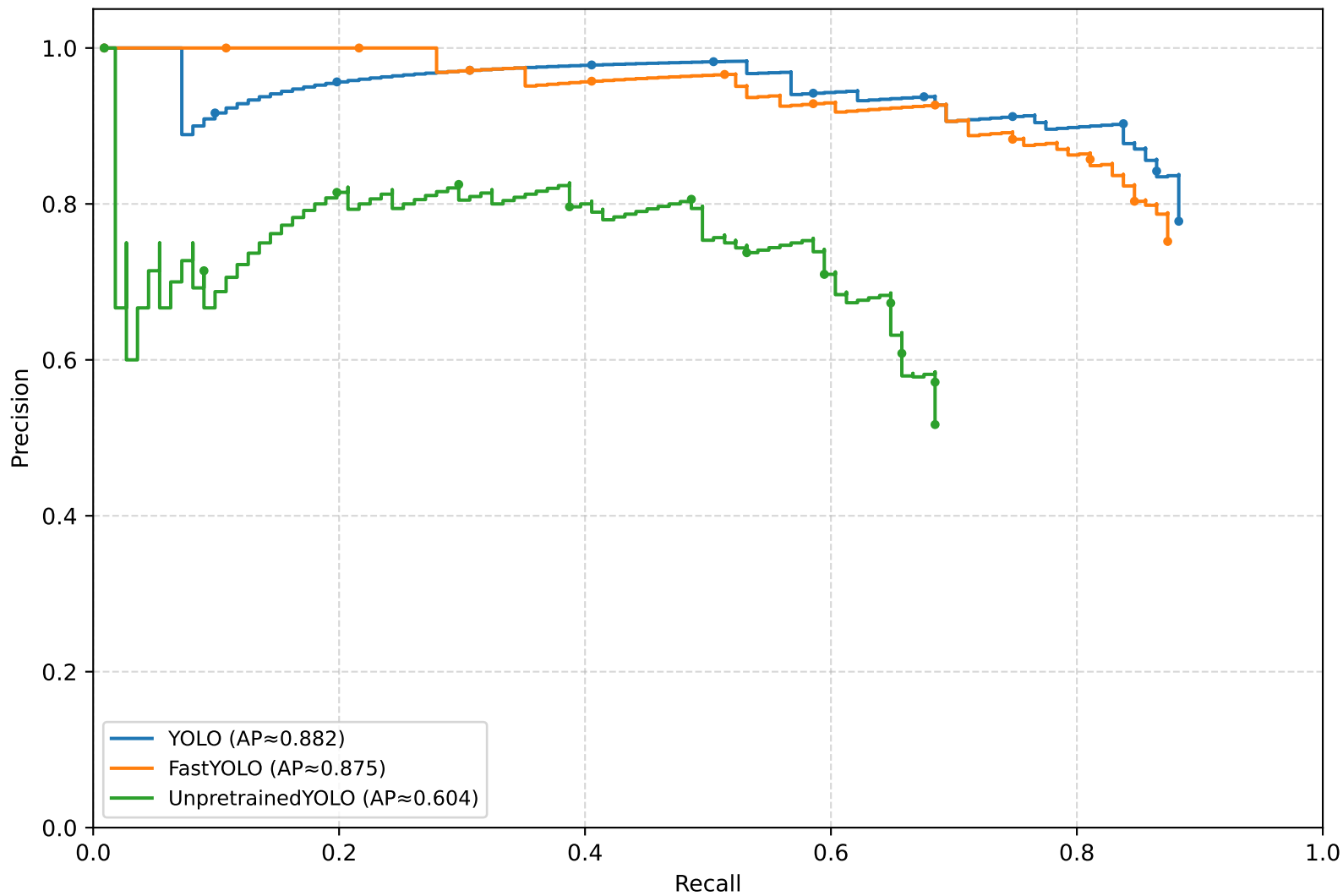
Precision — Recall curves at IoU = 0.75 (AP = area under PR curve)
