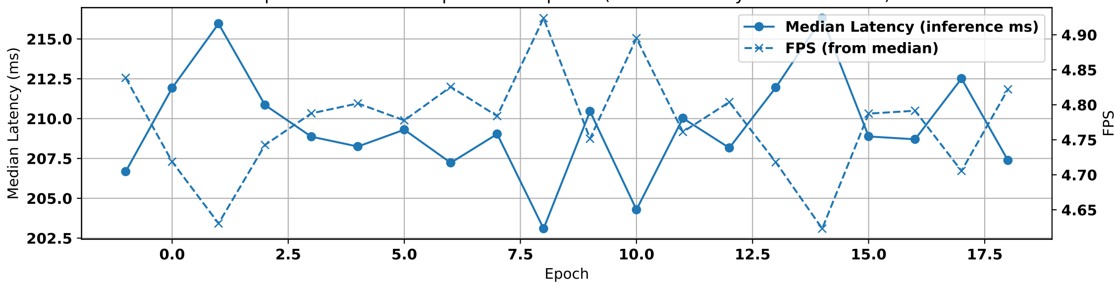
UnpretrainedYOLO — Speed over Epochs (median latency = inference ms)
