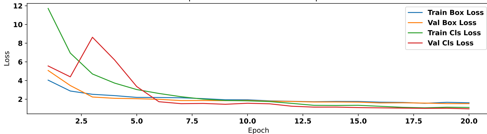
UnpretrainedYOLO — Metrics over Epochs
