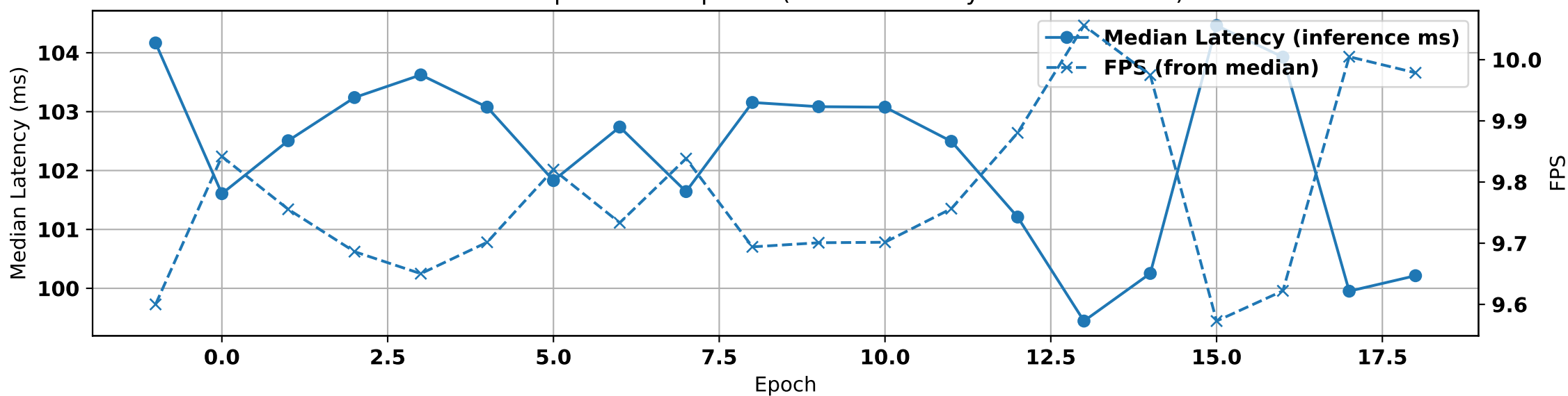
FastYOLO — Speed over Epochs (median latency = inference ms)
