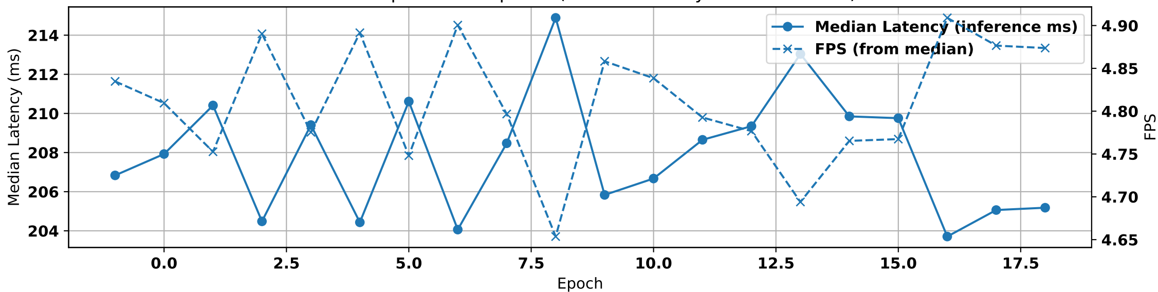
YOLO — Speed over Epochs (median latency = inference ms)
