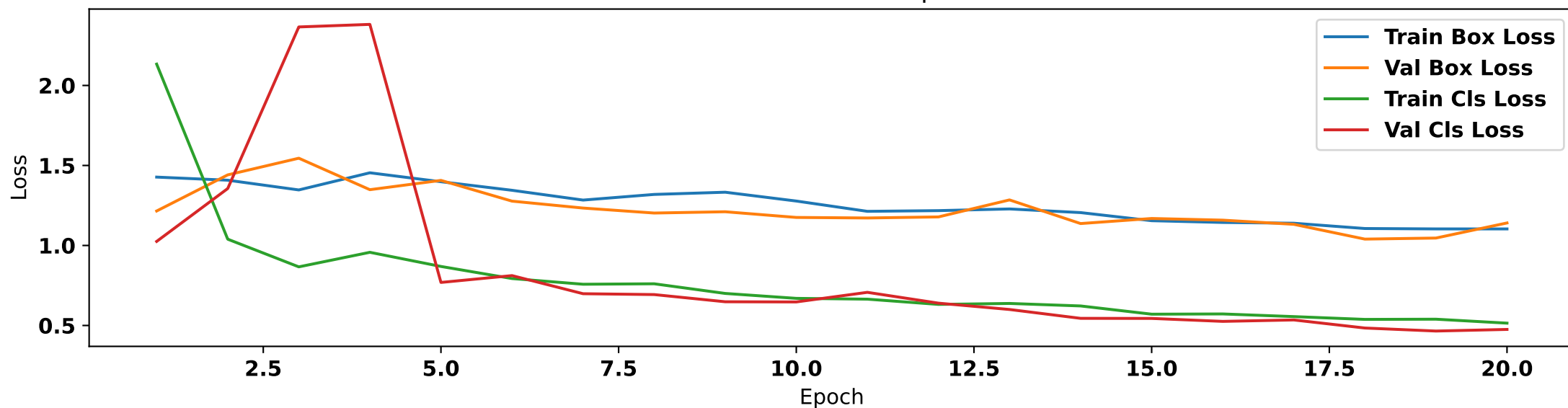
YOLO — Metrics over Epochs
