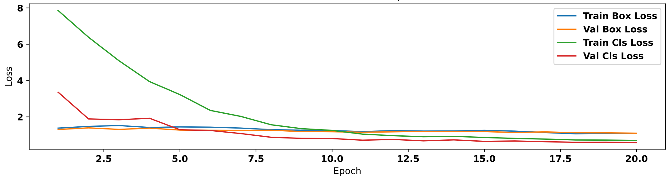
FastYOLO — Metrics over Epochs
