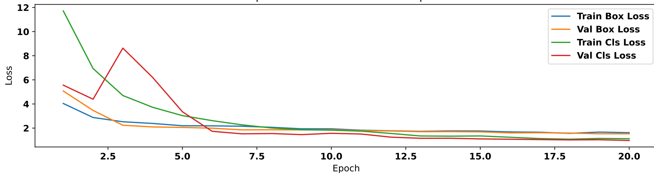
UnpretrainedYOLO — Metrics over Epochs
