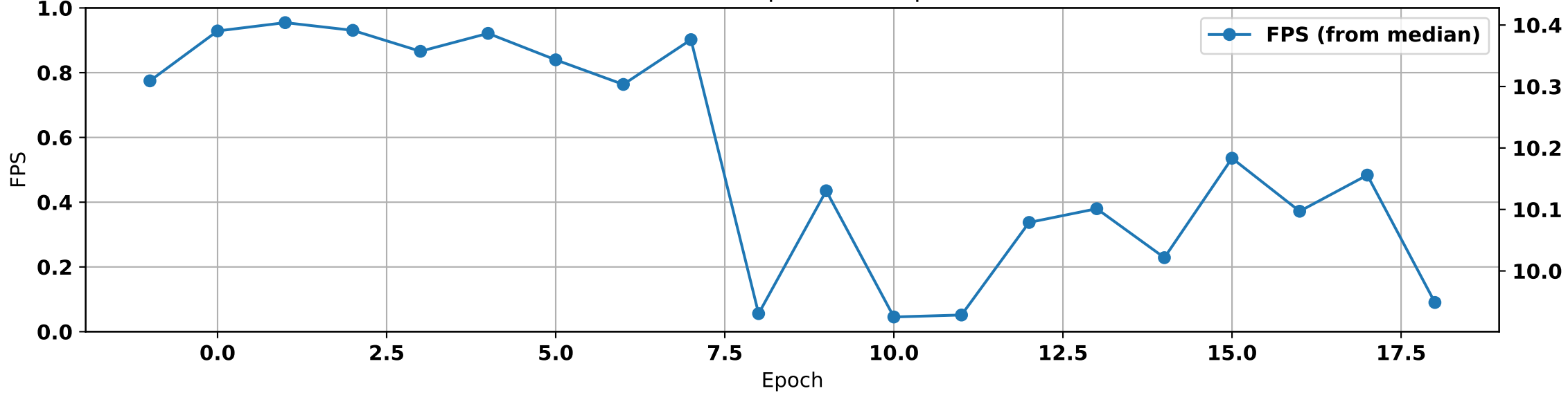
FastYOLO — Speed over Epochs
