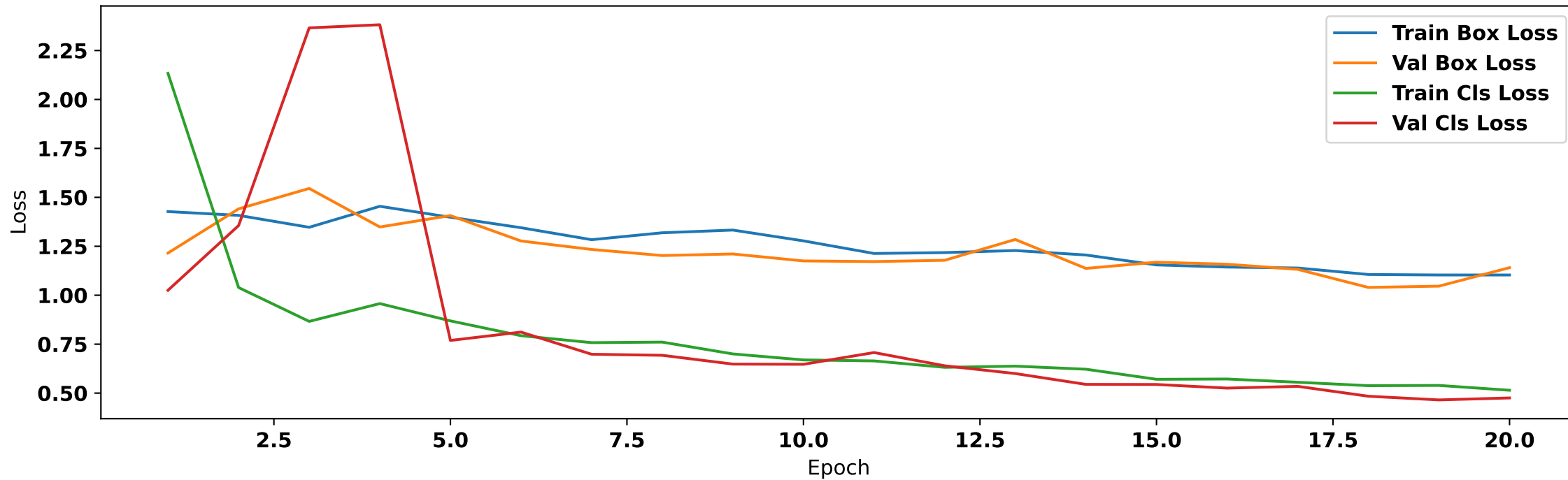
YOLO — Metrics over Epochs
