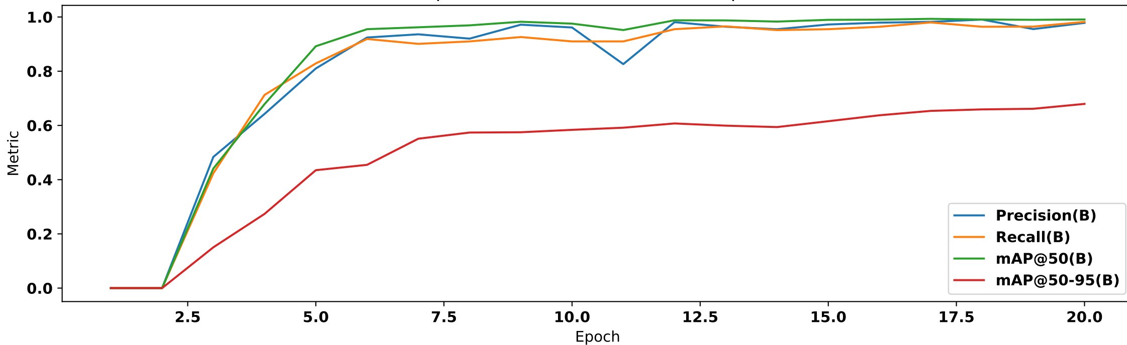
UnpretrainedYOLO — Metrics over Epochs
