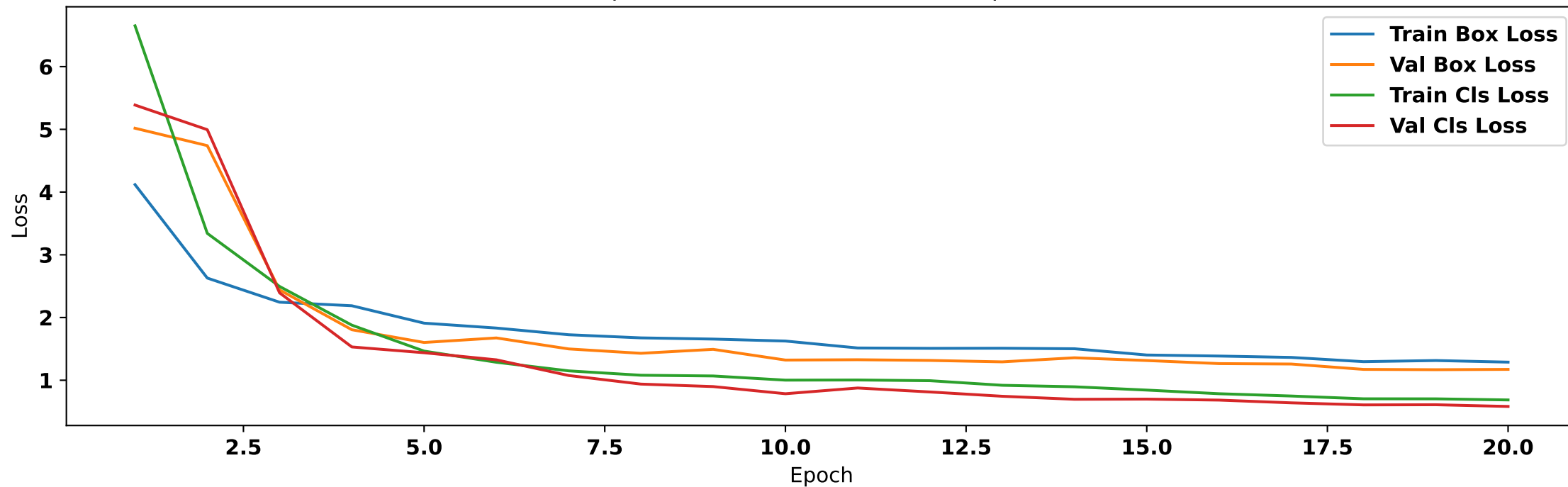
UnpretrainedYOLO — Metrics over Epochs
