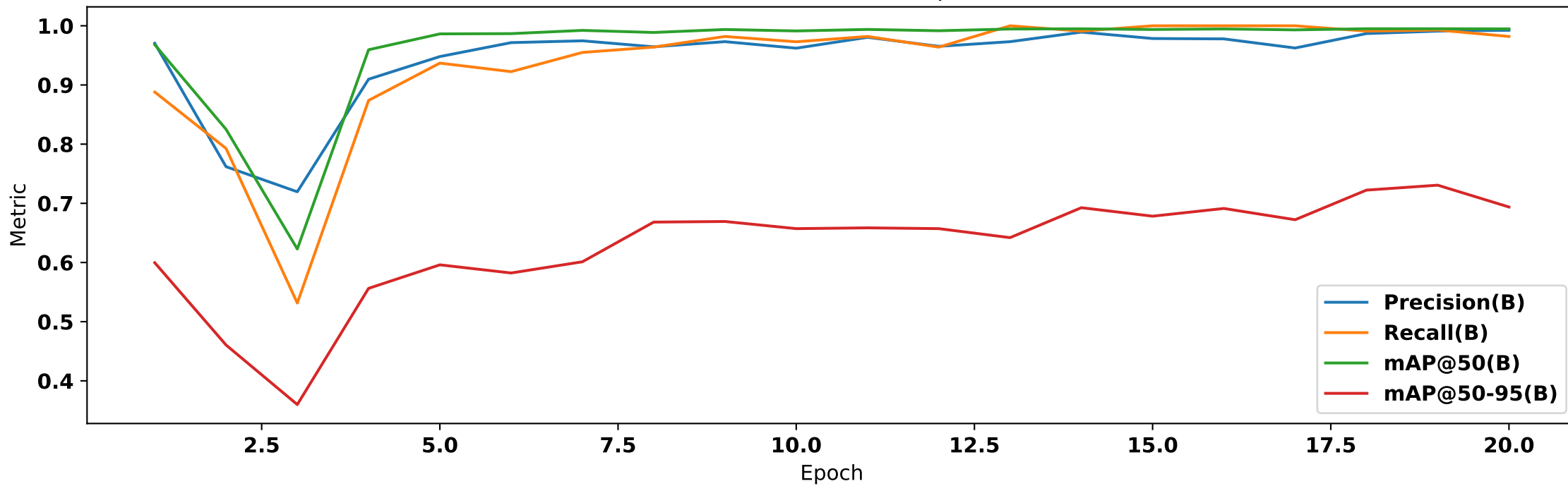
YOLO — Metrics over Epochs
