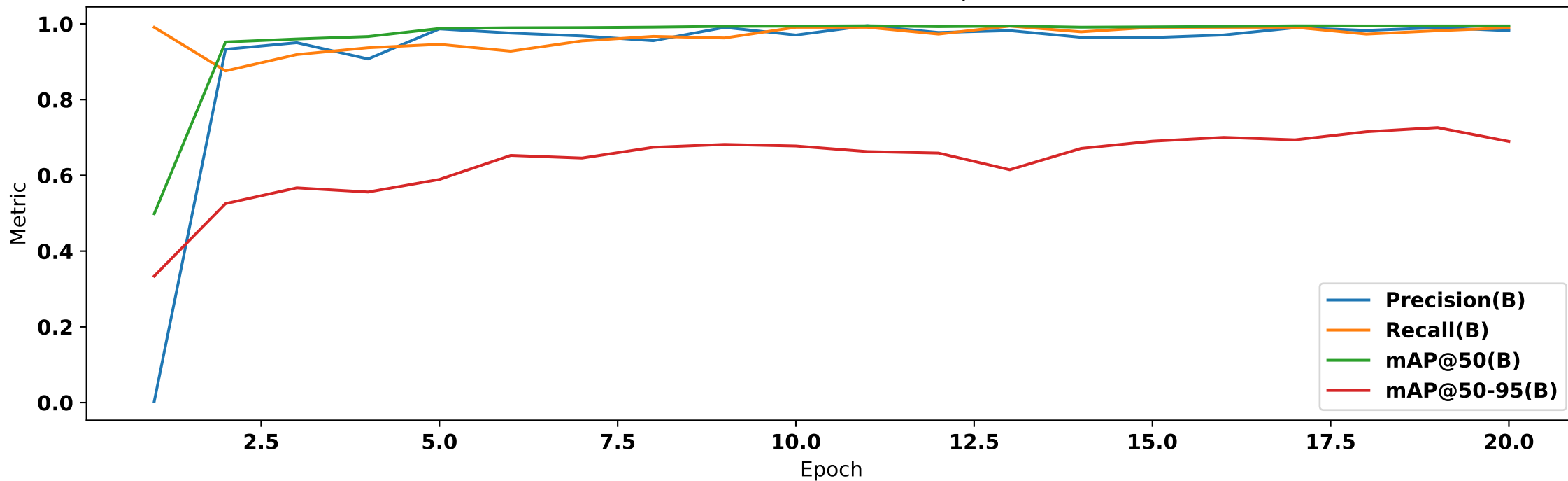
FastYOLO — Metrics over Epochs
