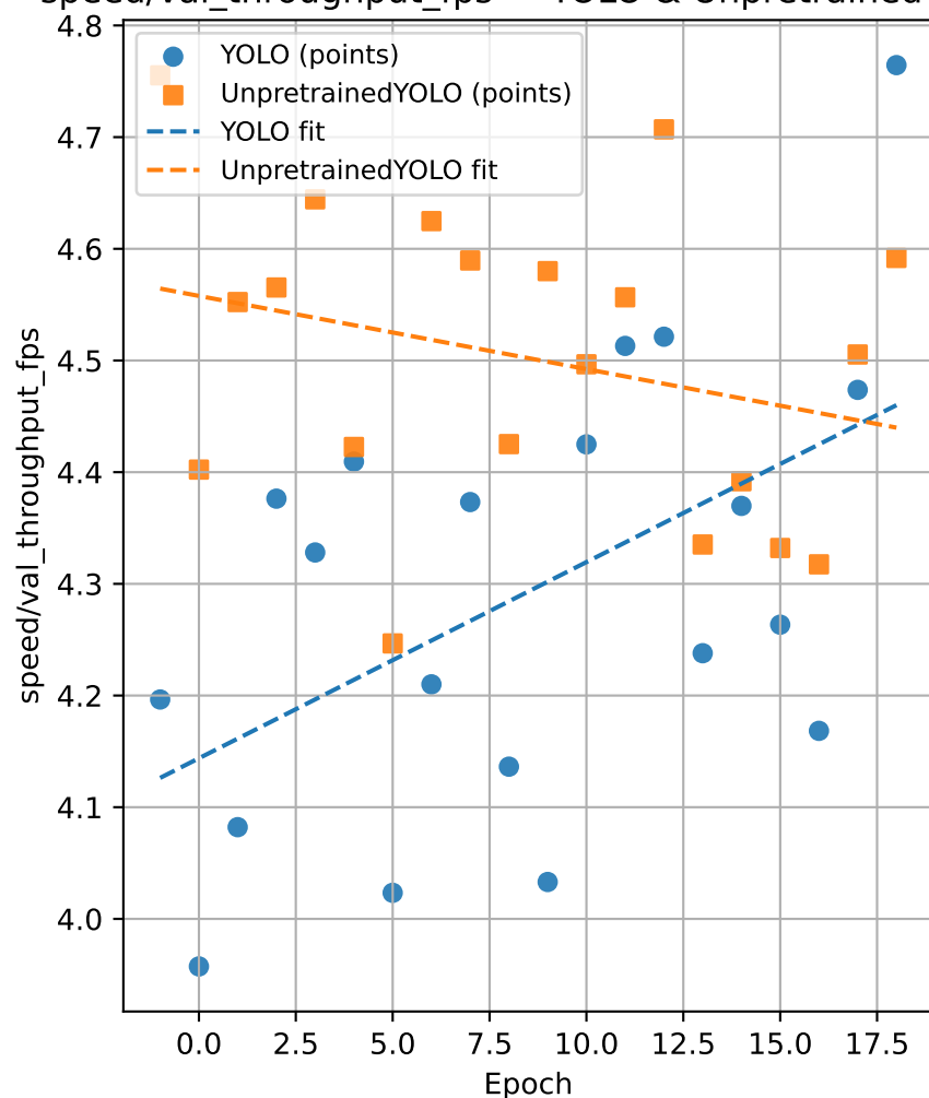
speed/val_throughput_fps — YOLO & UnpretrainedYOLO
