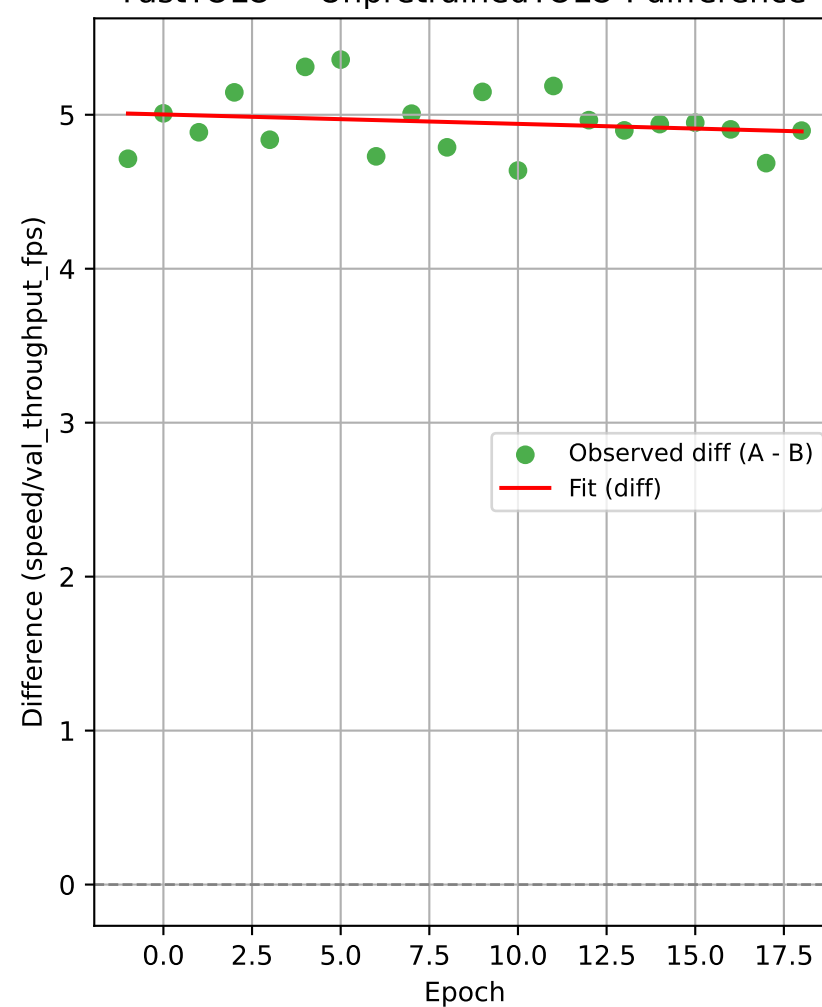
FastYOLO — UnpretrainedYOLO : difference
