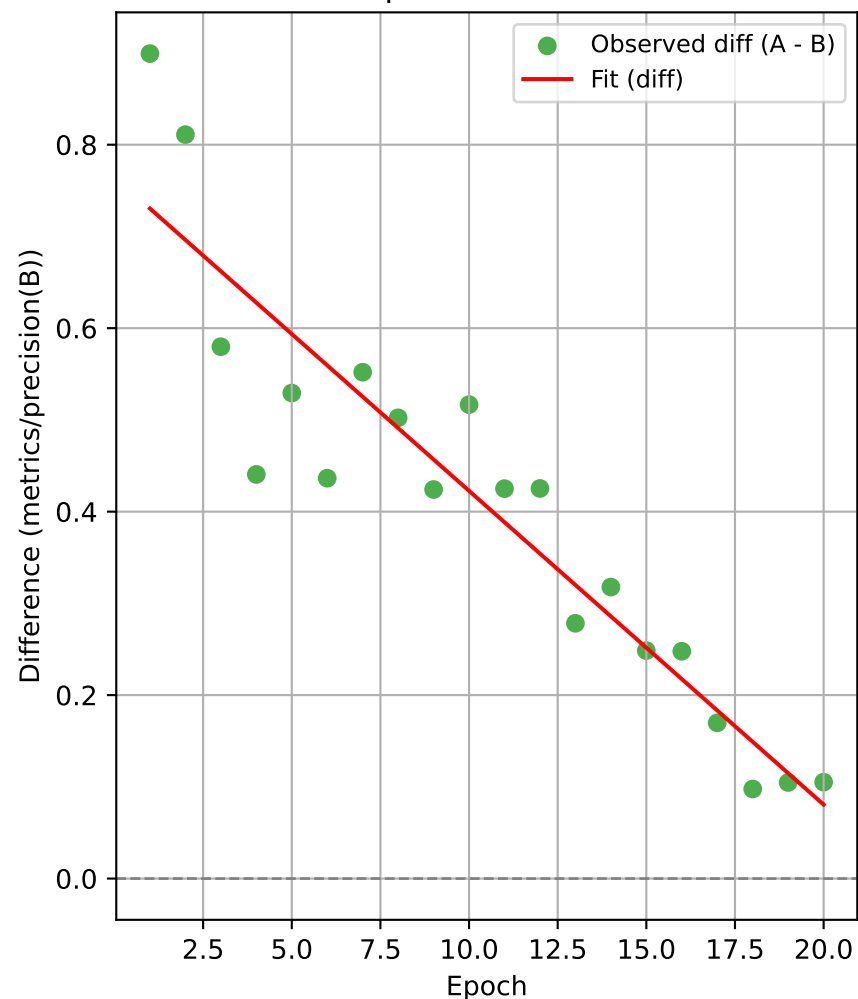
FastYOLO — UnpretrainedYOLO : difference
