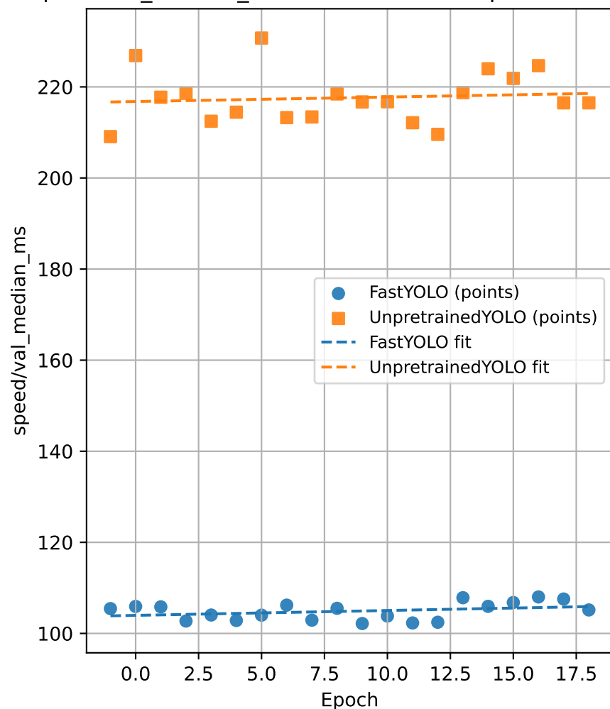
speed/val_median_ms — FastYOLO & UnpretrainedYOLO
