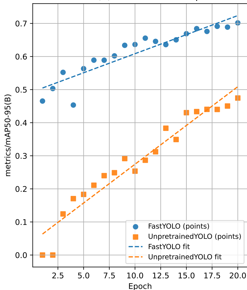
metrics/mAP50-95(B) — FastYOLO & UnpretrainedYOLO
