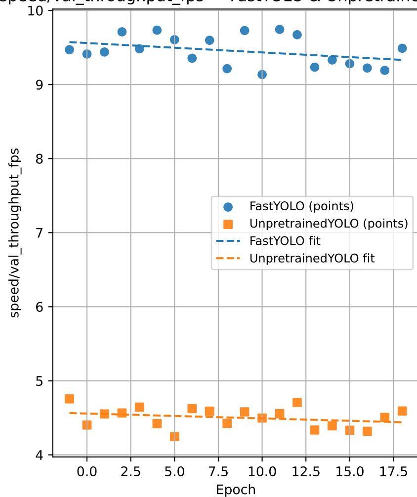
speed/val_throughput_fps — FastYOLO & UnpretrainedYOLO
