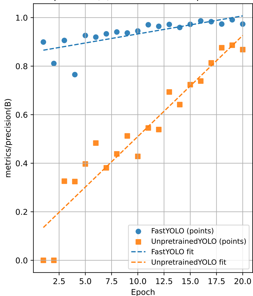
metrics/precision(B) — FastYOLO & UnpretrainedYOLO
