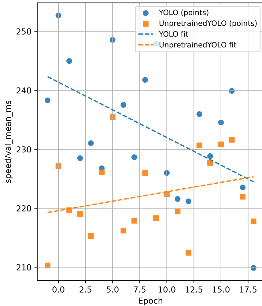
speed/val_mean_ms — YOLO & UnpretrainedYOLO
