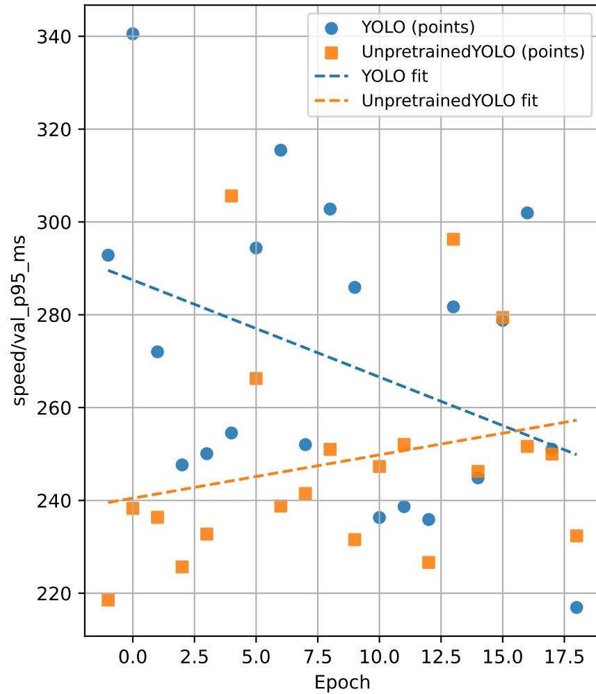
speed/val_p95_ms — YOLO & UnpretrainedYOLO
